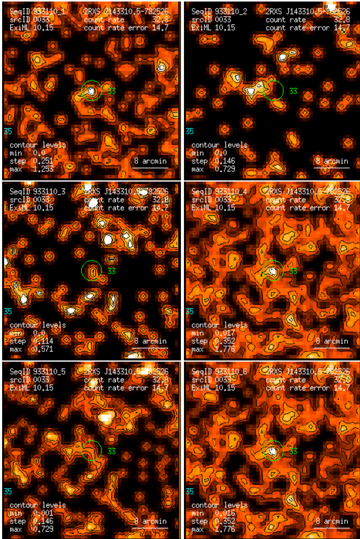
Figure 33: RASS 933110: detection 0033: band rate images, Gaussian filter: (1) PSPC channels 11 – 41, (2) 52 – 90, (3) 91 – 201, (4) 11 – 235, (5) 52 – 201, (6) 11 – 201. Broad band rates in counts/ks. Band rate contour levels in counts/ks/arcmin 2 .
