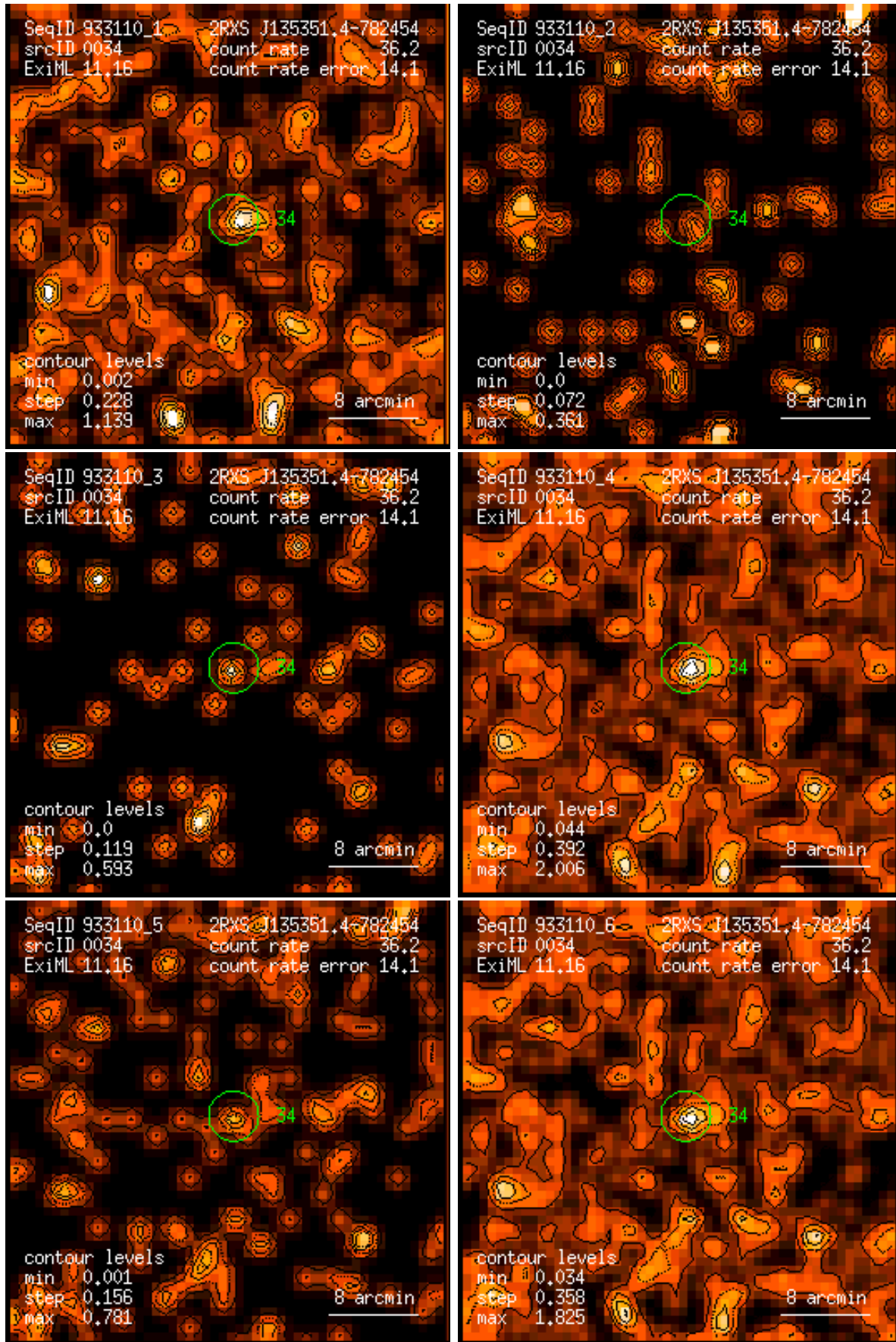
Figure 34: RASS 933110: detection 0034: band rate images, Gaussian filter: (1) PSPC channels 11 – 41, (2) 52 – 90, (3) 91 – 201, (4) 11 – 235, (5) 52 – 201, (6) 11 – 201. Broad band rates in counts/ks. Band rate contour levels in counts/ks/arcmin 2 .
