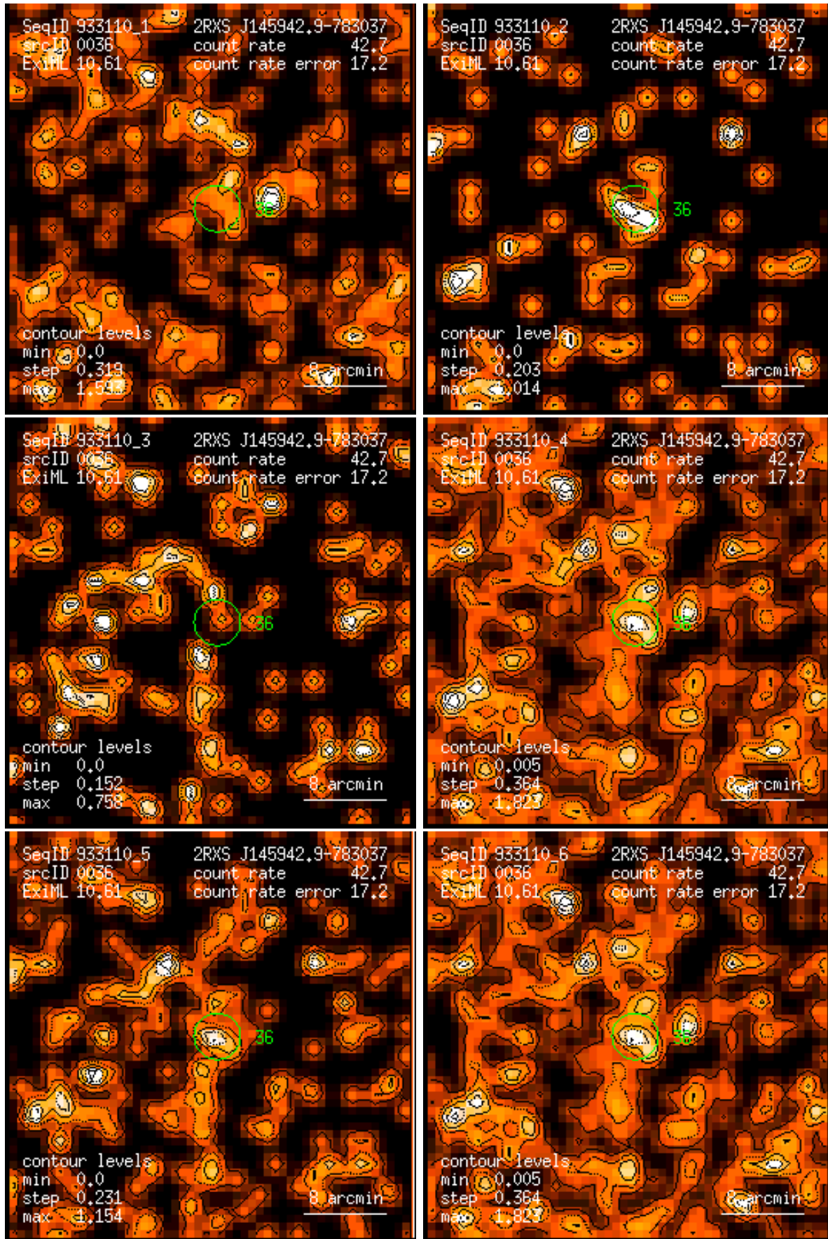
Figure 36: RASS 933110: detection 0036: band rate images, Gaussian filter: (1) PSPC channels 11 – 41, (2) 52 – 90, (3) 91 – 201, (4) 11 – 235, (5) 52 – 201, (6) 11 – 201. Broad band rates in counts/ks. Band rate contour levels in counts/ks/arcmin 2 .
