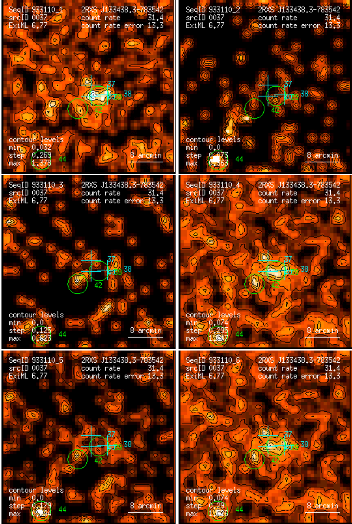
Figure 37: RASS 933110: detection 0037: band rate images, Gaussian filter: (1) PSPC channels 11 – 41, (2) 52 – 90, (3) 91 – 201, (4) 11 – 235, (5) 52 – 201, (6) 11 – 201. Broad band rates in counts/ks. Band rate contour levels in counts/ks/arcmin 2 .
