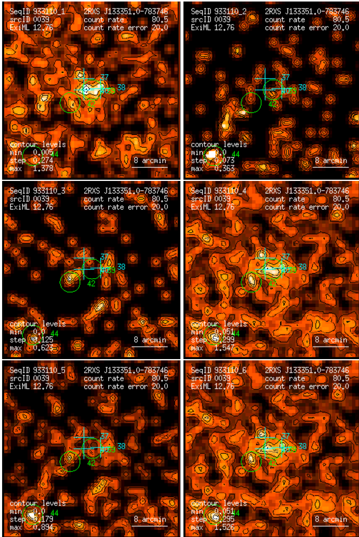
Figure 39: RASS 933110: detection 0039: band rate images, Gaussian filter: (1) PSPC channels 11 – 41, (2) 52 – 90, (3) 91 – 201, (4) 11 – 235, (5) 52 – 201, (6) 11 – 201. Broad band rates in counts/ks. Band rate contour levels in counts/ks/arcmin 2 .
