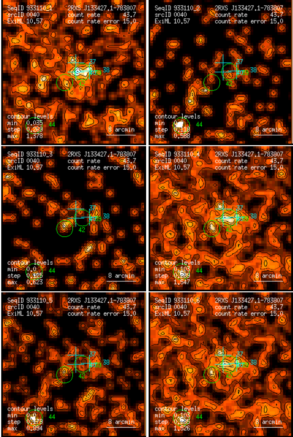
Figure 40: RASS 933110: detection 0040: band rate images, Gaussian filter: (1) PSPC channels 11 – 41, (2) 52 – 90, (3) 91 – 201, (4) 11 – 235, (5) 52 – 201, (6) 11 – 201. Broad band rates in counts/ks. Band rate contour levels in counts/ks/arcmin 2 .
