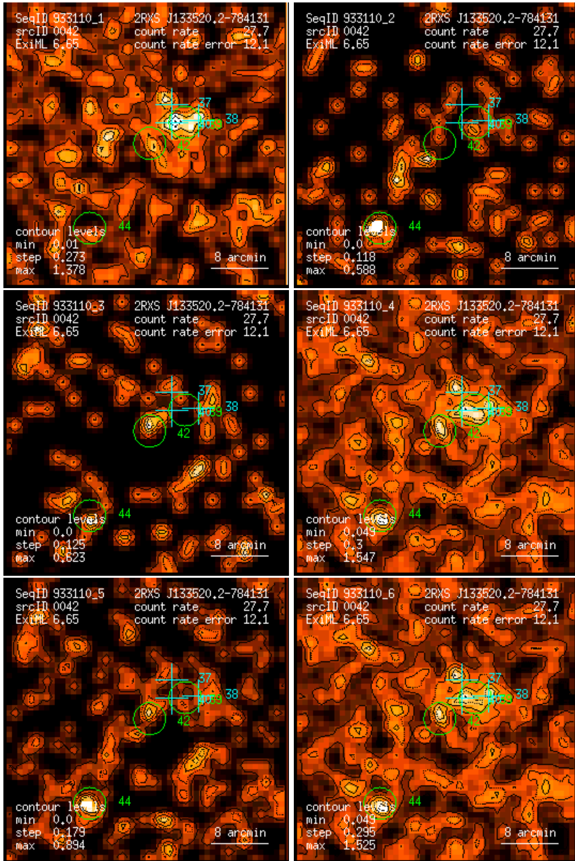
Figure 42: RASS 933110: detection 0042: band rate images, Gaussian filter: (1) PSPC channels 11 – 41, (2) 52 – 90, (3) 91 – 201, (4) 11 – 235, (5) 52 – 201, (6) 11 – 201. Broad band rates in counts/ks. Band rate contour levels in counts/ks/arcmin 2 .
