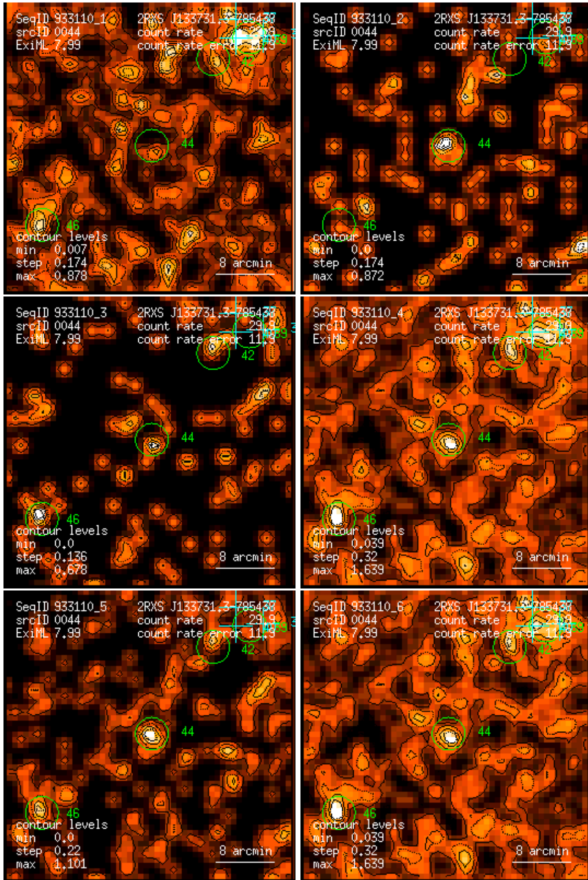
Figure 44: RASS 933110: detection 0044: band rate images, Gaussian filter: (1) PSPC channels 11 – 41, (2) 52 – 90, (3) 91 – 201, (4) 11 – 235, (5) 52 – 201, (6) 11 – 201. Broad band rates in counts/ks. Band rate contour levels in counts/ks/arcmin 2 .
