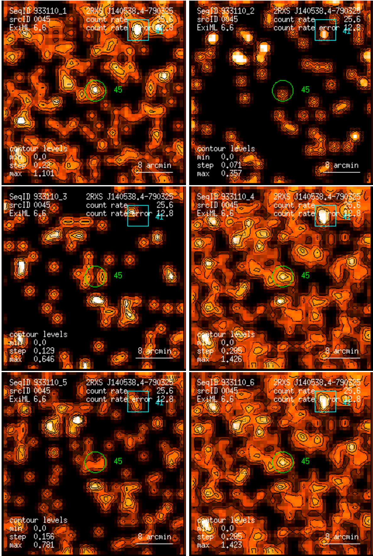
Figure 45: RASS 933110: detection 0045: band rate images, Gaussian filter: (1) PSPC channels 11 – 41, (2) 52 – 90, (3) 91 – 201, (4) 11 – 235, (5) 52 – 201, (6) 11 – 201. Broad band rates in counts/ks. Band rate contour levels in counts/ks/arcmin 2 .
