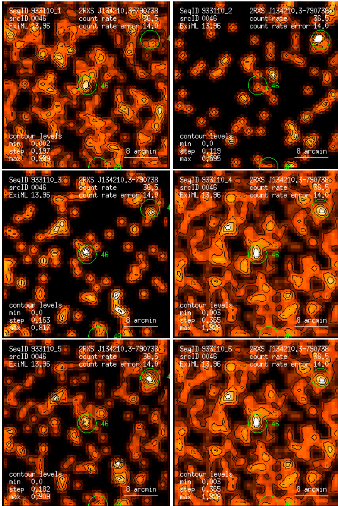
Figure 46: RASS 933110: detection 0046: band rate images, Gaussian filter: (1) PSPC channels 11 – 41, (2) 52 – 90, (3) 91 – 201, (4) 11 – 235, (5) 52 – 201, (6) 11 – 201. Broad band rates in counts/ks. Band rate contour levels in counts/ks/arcmin 2 .
