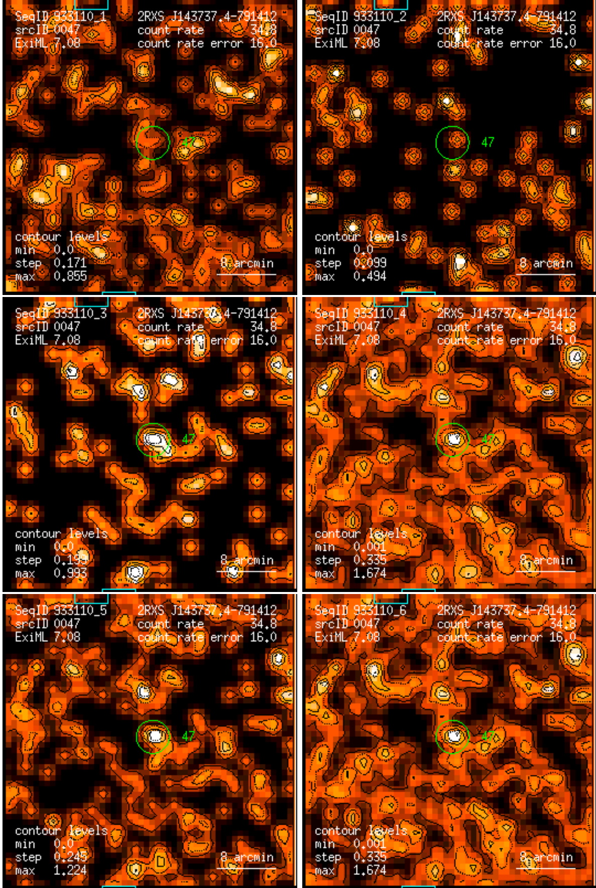
Figure 47: RASS 933110: detection 0047: band rate images, Gaussian filter: (1) PSPC channels 11 – 41, (2) 52 – 90, (3) 91 – 201, (4) 11 – 235, (5) 52 – 201, (6) 11 – 201. Broad band rates in counts/ks. Band rate contour levels in counts/ks/arcmin 2 .
