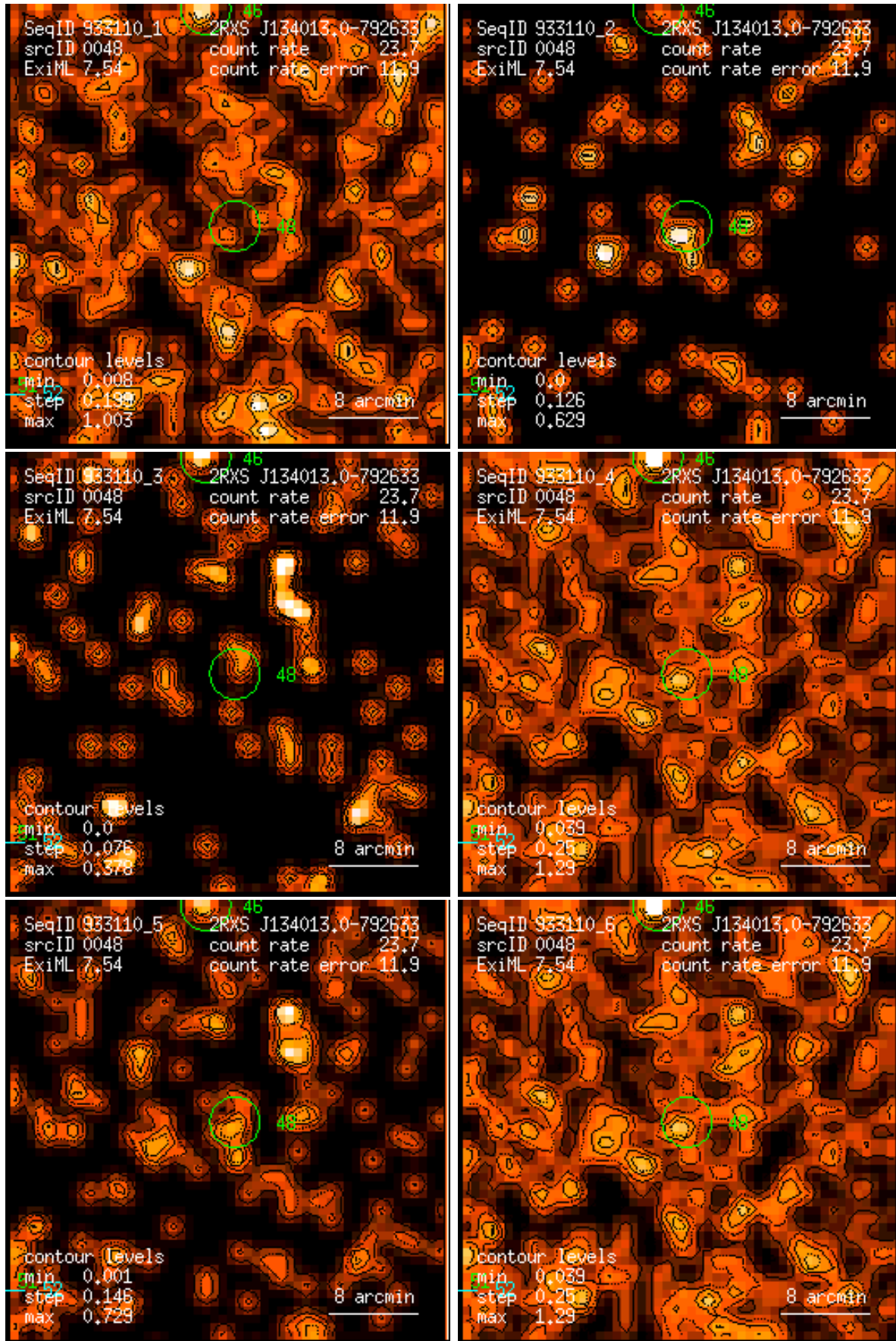
Figure 48: RASS 933110: detection 0048: band rate images, Gaussian filter: (1) PSPC channels 11 – 41, (2) 52 – 90, (3) 91 – 201, (4) 11 – 235, (5) 52 – 201, (6) 11 – 201. Broad band rates in counts/ks. Band rate contour levels in counts/ks/arcmin 2 .
