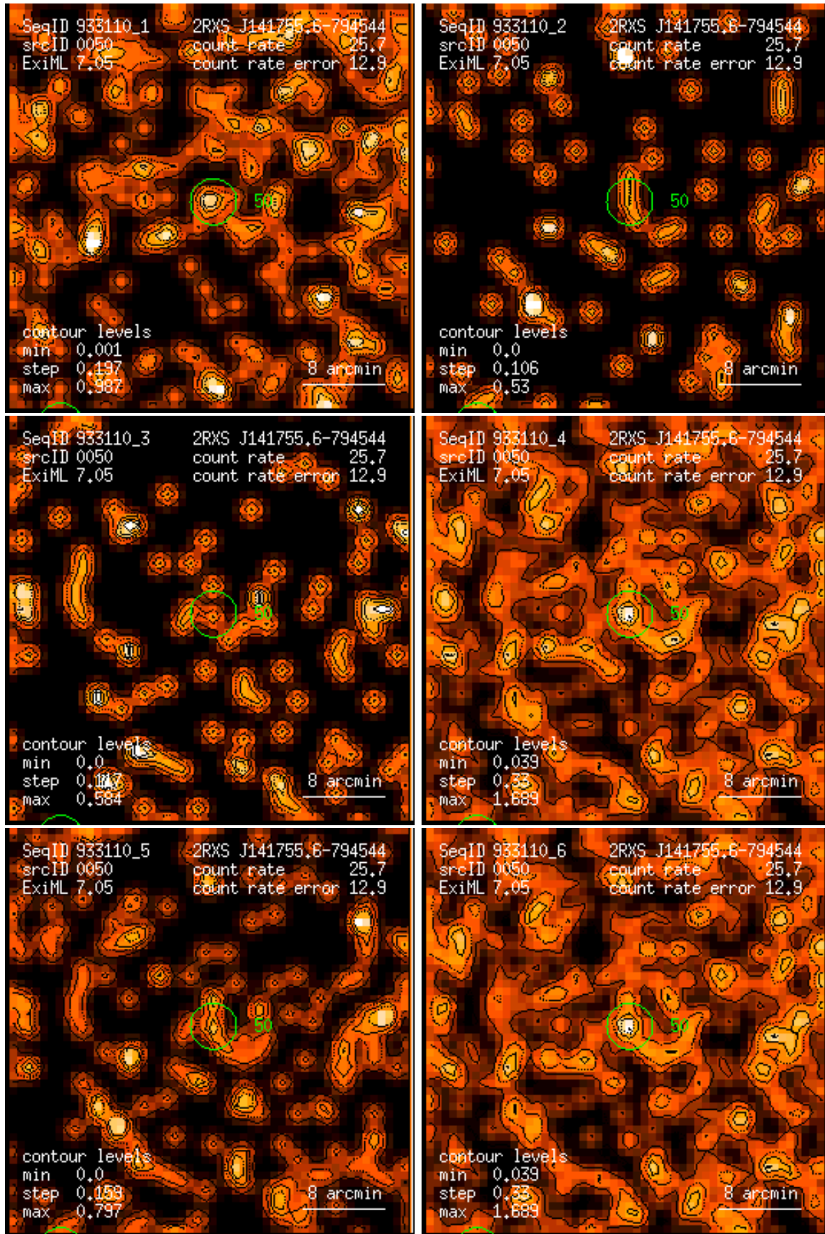
Figure 50: RASS 933110: detection 0050: band rate images, Gaussian filter: (1) PSPC channels 11 – 41, (2) 52 – 90, (3) 91 – 201, (4) 11 – 235, (5) 52 – 201, (6) 11 – 201. Broad band rates in counts/ks. Band rate contour levels in counts/ks/arcmin 2 .
