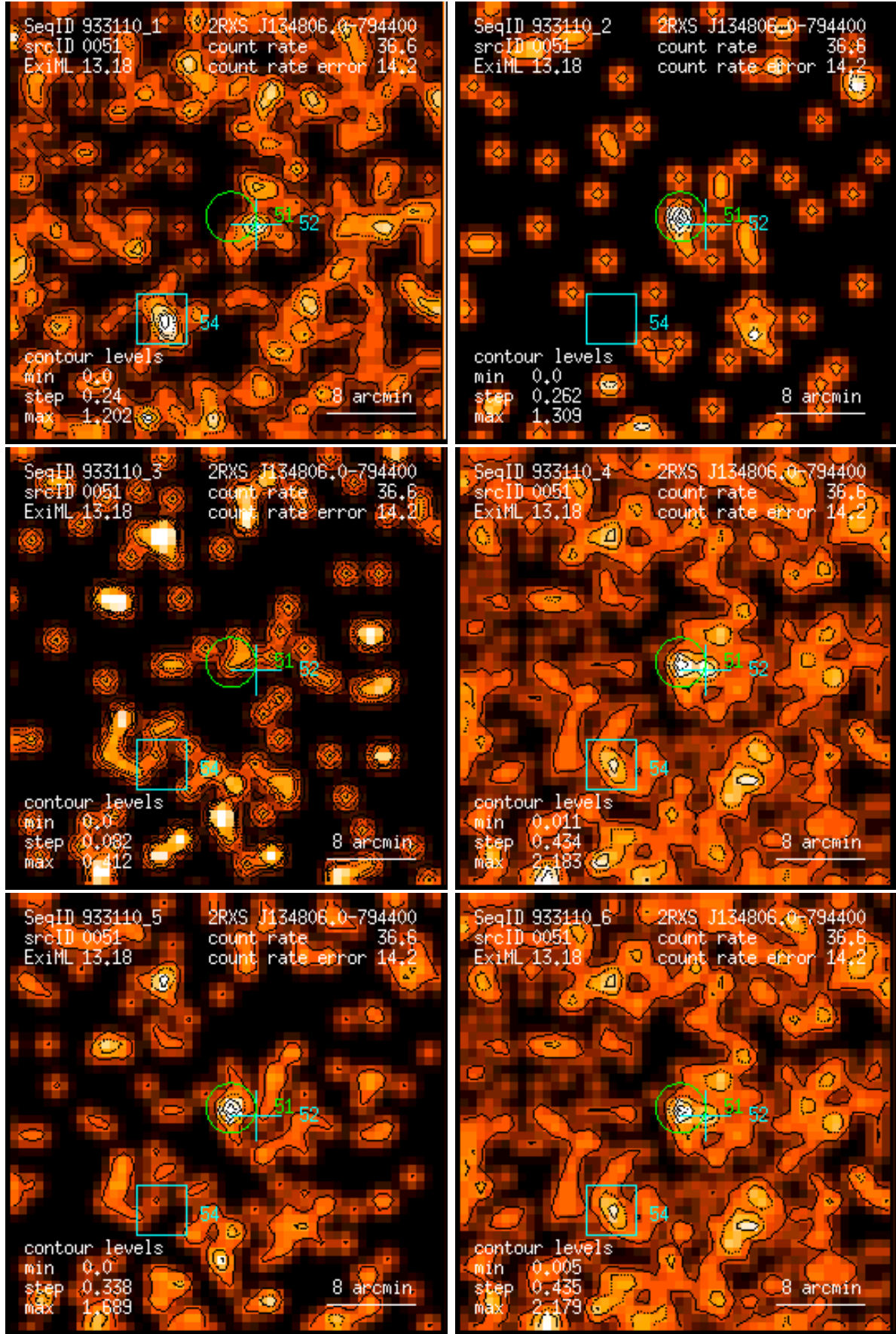
Figure 51: RASS 933110: detection 0051: band rate images, Gaussian filter: (1) PSPC channels 11 – 41, (2) 52 – 90, (3) 91 – 201, (4) 11 – 235, (5) 52 – 201, (6) 11 – 201. Broad band rates in counts/ks. Band rate contour levels in counts/ks/arcmin 2 .
