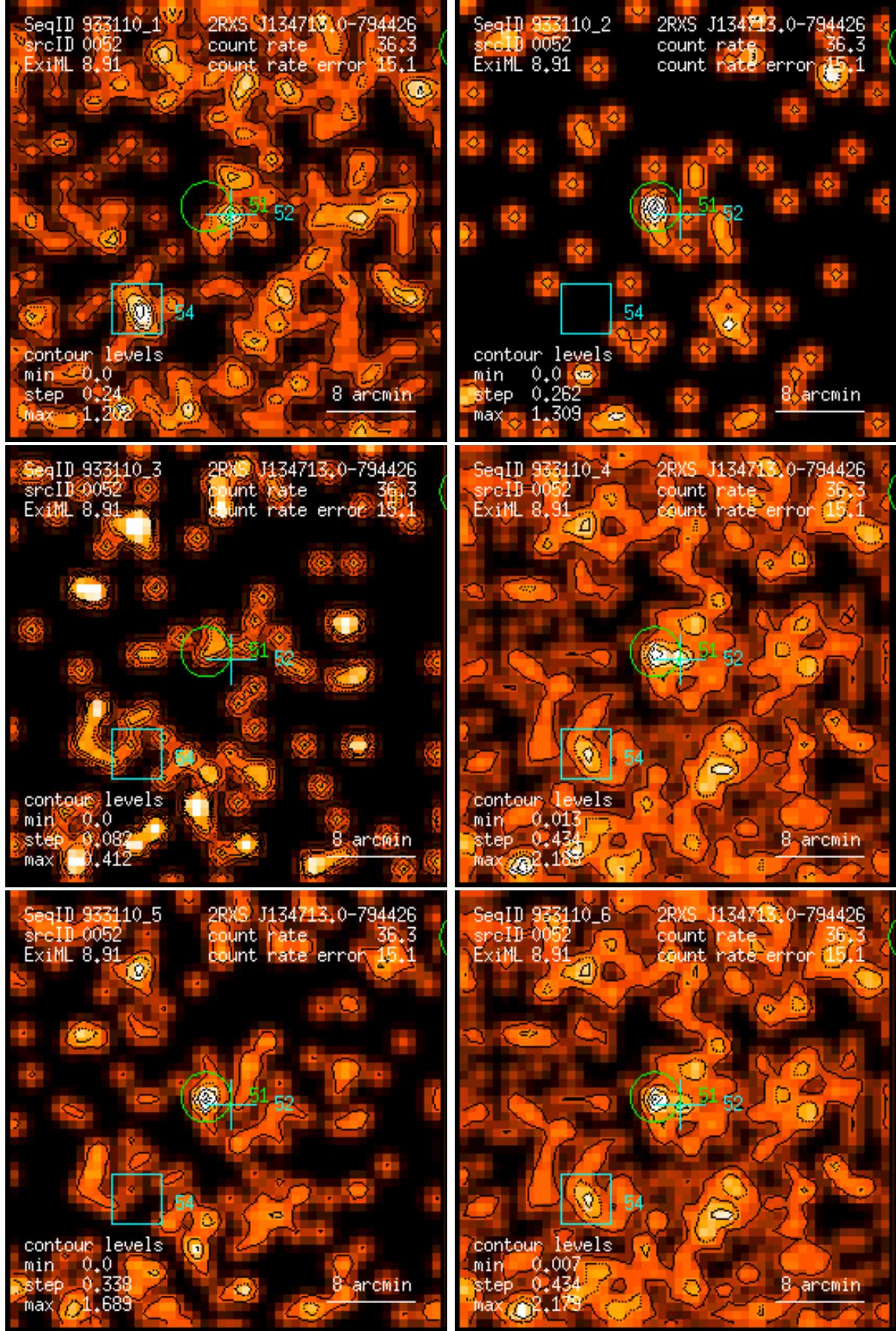
Figure 52: RASS 933110: detection 0052: band rate images, Gaussian filter: (1) PSPC channels 11 – 41, (2) 52 – 90, (3) 91 – 201, (4) 11 – 235, (5) 52 – 201, (6) 11 – 201. Broad band rates in counts/ks. Band rate contour levels in counts/ks/arcmin 2 .
