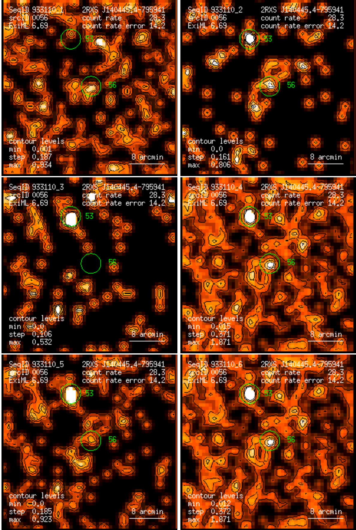
Figure 56: RASS 933110: detection 0056: band rate images, Gaussian filter: (1) PSPC channels 11 – 41, (2) 52 – 90, (3) 91 – 201, (4) 11 – 235, (5) 52 – 201, (6) 11 – 201. Broad band rates in counts/ks. Band rate contour levels in counts/ks/arcmin 2 .
