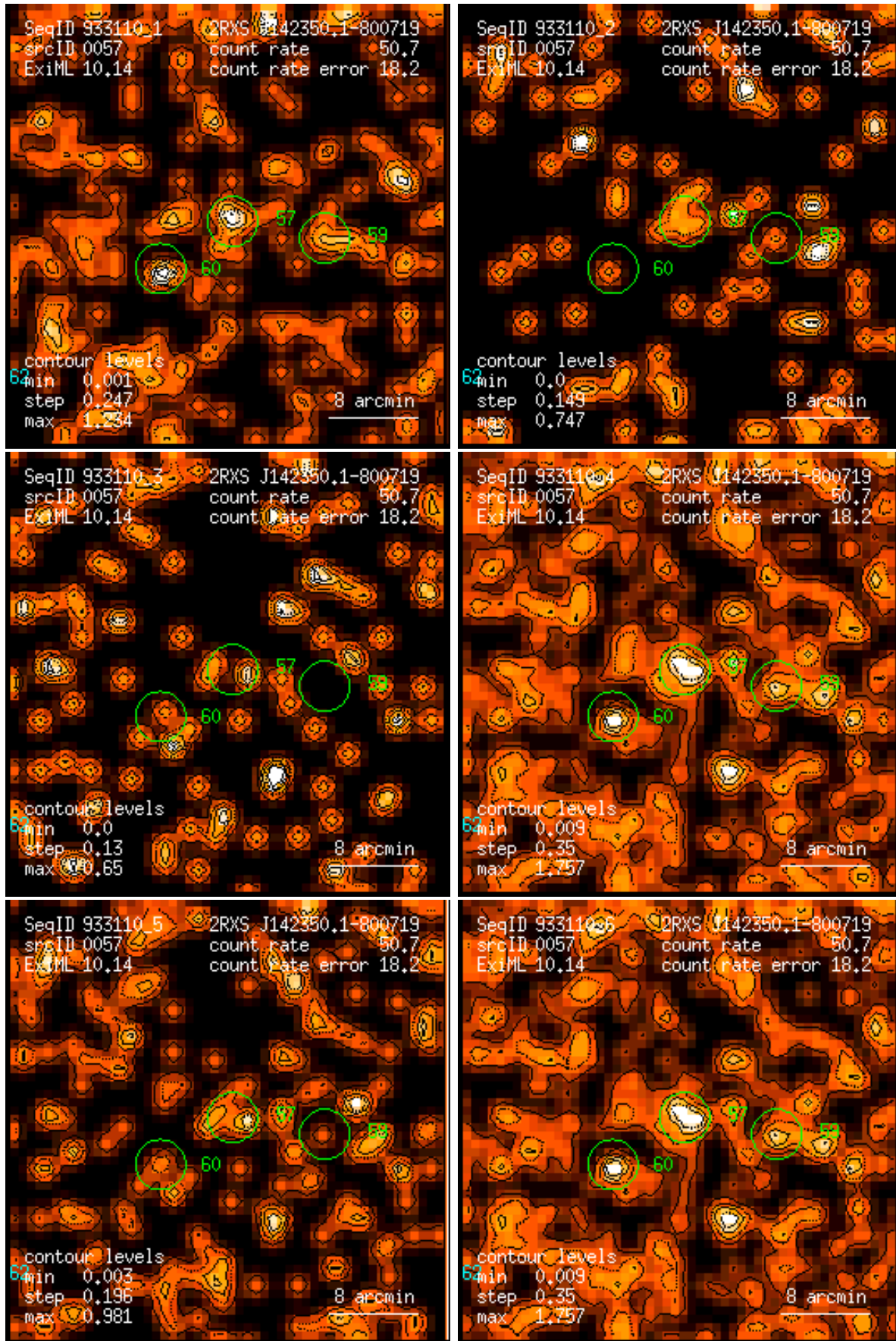
Figure 57: RASS 933110: detection 0057: band rate images, Gaussian filter: (1) PSPC channels 11 – 41, (2) 52 – 90, (3) 91 – 201, (4) 11 – 235, (5) 52 – 201, (6) 11 – 201. Broad band rates in counts/ks. Band rate contour levels in counts/ks/arcmin 2 .
