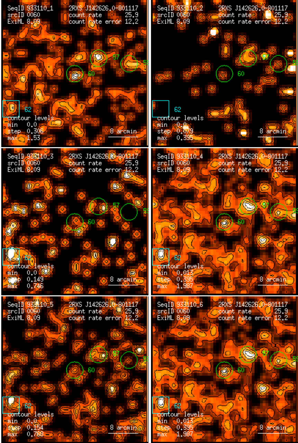
Figure 60: RASS 933110: detection 0060: band rate images, Gaussian filter: (1) PSPC channels 11 – 41, (2) 52 – 90, (3) 91 – 201, (4) 11 – 235, (5) 52 – 201, (6) 11 – 201. Broad band rates in counts/ks. Band rate contour levels in counts/ks/arcmin 2 .
