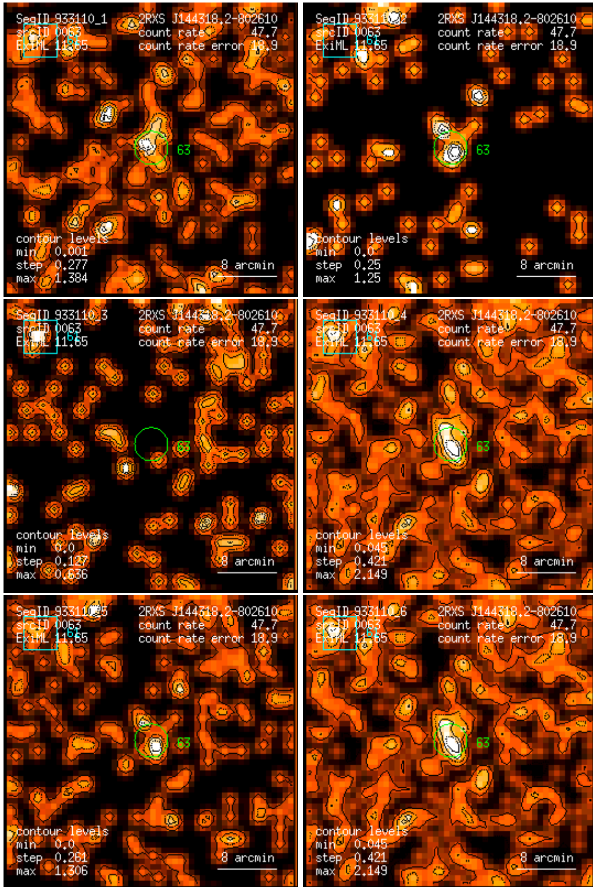
Figure 63: RASS 933110: detection 0063: band rate images, Gaussian filter: (1) PSPC channels 11 – 41, (2) 52 – 90, (3) 91 – 201, (4) 11 – 235, (5) 52 – 201, (6) 11 – 201. Broad band rates in counts/ks. Band rate contour levels in counts/ks/arcmin 2 .
