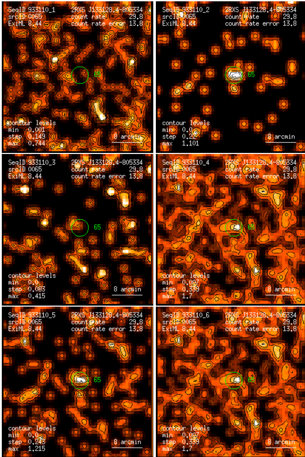
Figure 65: RASS 933110: detection 0065: band rate images, Gaussian filter: (1) PSPC channels 11 – 41, (2) 52 – 90, (3) 91 – 201, (4) 11 – 235, (5) 52 – 201, (6) 11 – 201. Broad band rates in counts/ks. Band rate contour levels in counts/ks/arcmin 2 .
