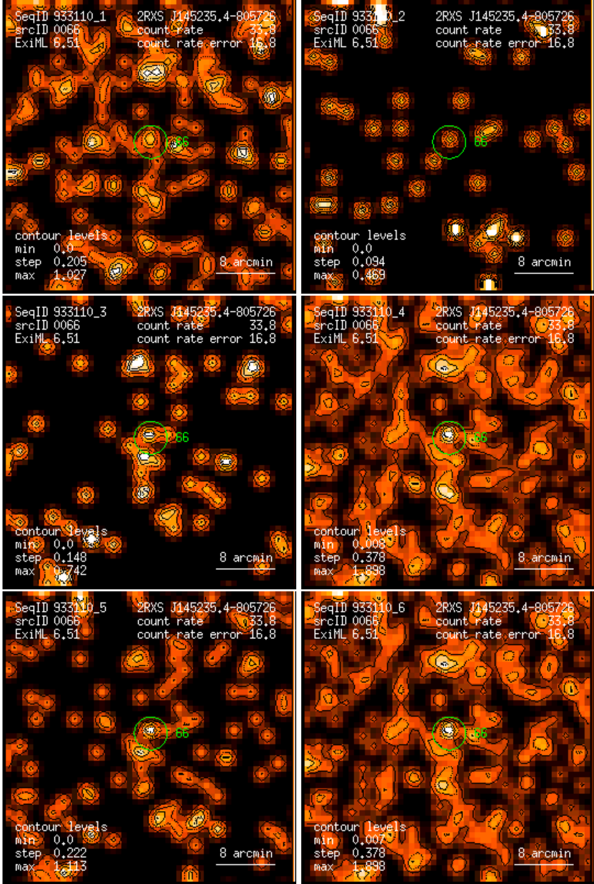
Figure 66: RASS 933110: detection 0066: band rate images, Gaussian filter: (1) PSPC channels 11 – 41, (2) 52 – 90, (3) 91 – 201, (4) 11 – 235, (5) 52 – 201, (6) 11 – 201. Broad band rates in counts/ks. Band rate contour levels in counts/ks/arcmin 2 .
