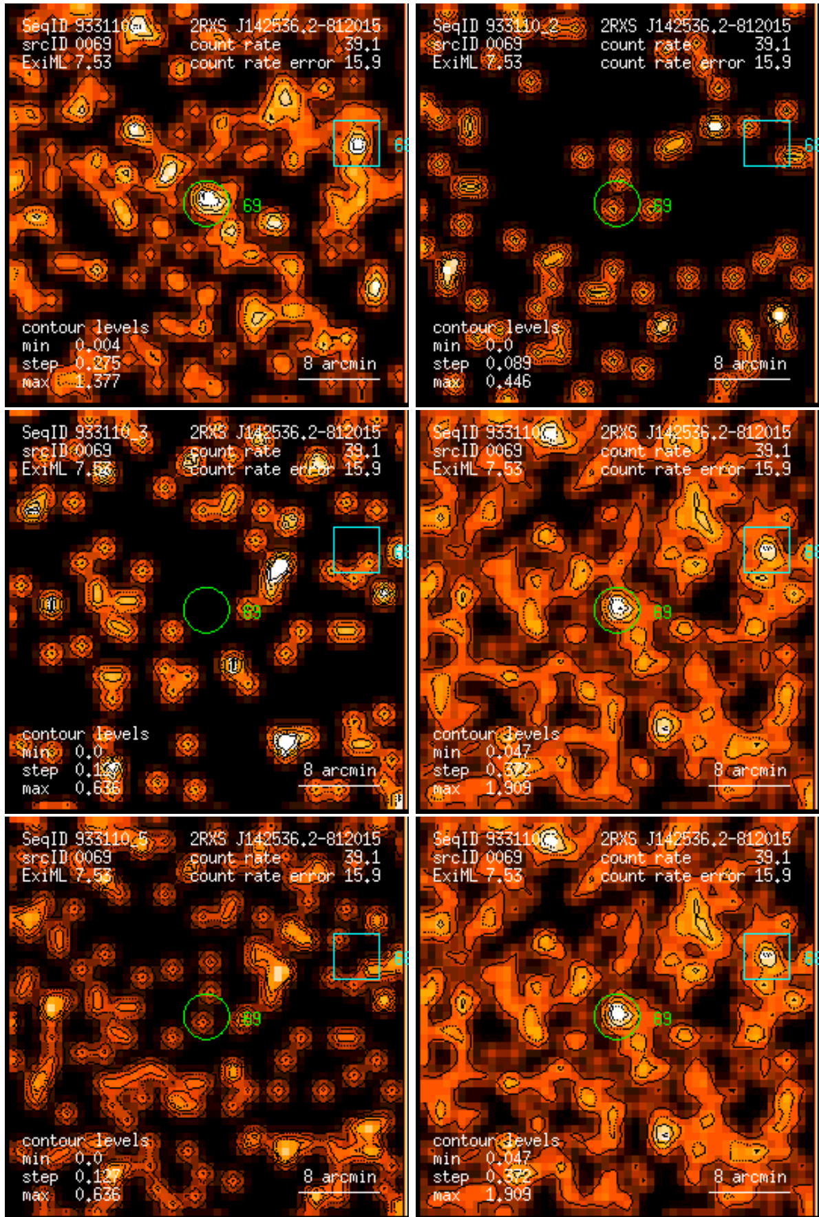
Figure 69: RASS 933110: detection 0069: band rate images, Gaussian filter: (1) PSPC channels 11 – 41, (2) 52 – 90, (3) 91 – 201, (4) 11 – 235, (5) 52 – 201, (6) 11 – 201. Broad band rates in counts/ks. Band rate contour levels in counts/ks/arcmin 2 .
