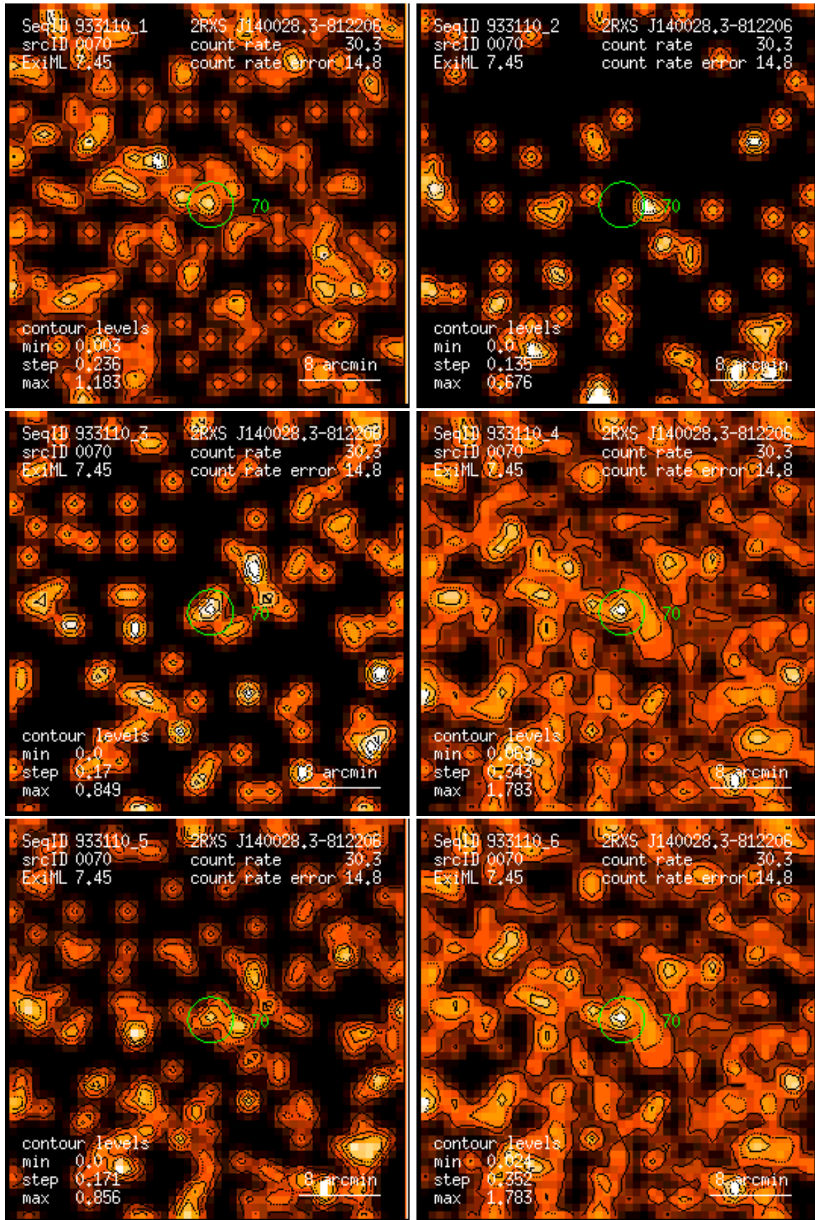
Figure 70: RASS 933110: detection 0070: band rate images, Gaussian filter: (1) PSPC channels 11 – 41, (2) 52 – 90, (3) 91 – 201, (4) 11 – 235, (5) 52 – 201, (6) 11 – 201. Broad band rates in counts/ks. Band rate contour levels in counts/ks/arcmin 2 .
