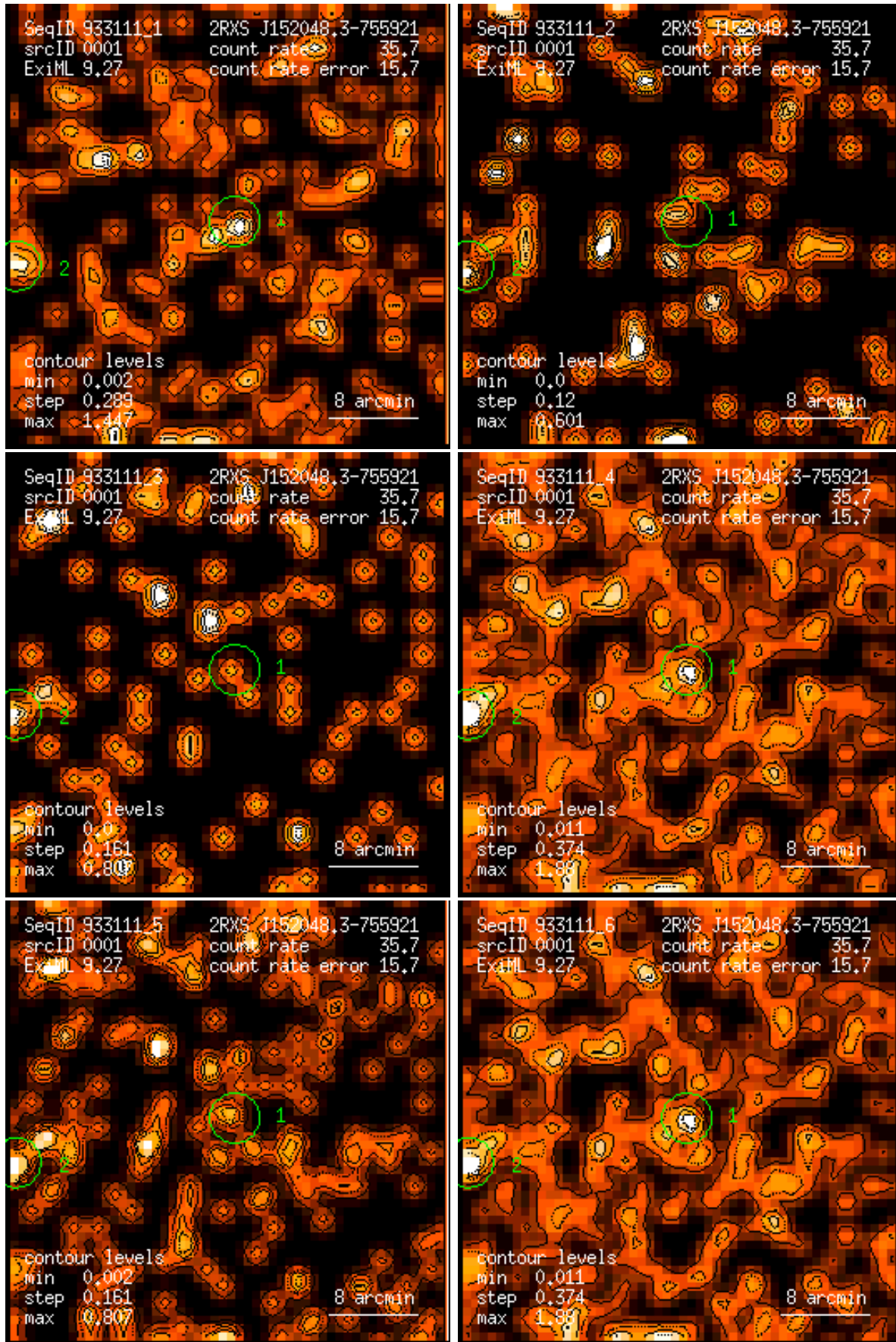
Figure 1: RASS 933111: detection 0001: band rate images, Gaussian filter: (1) PSPC channels 11 – 41, (2) 52 – 90, (3) 91 – 201, (4) 11 – 235, (5) 52 – 201, (6) 11 – 201. Broad band rates in counts/ks. Band rate contour levels in counts/ks/arcmin 2 .
