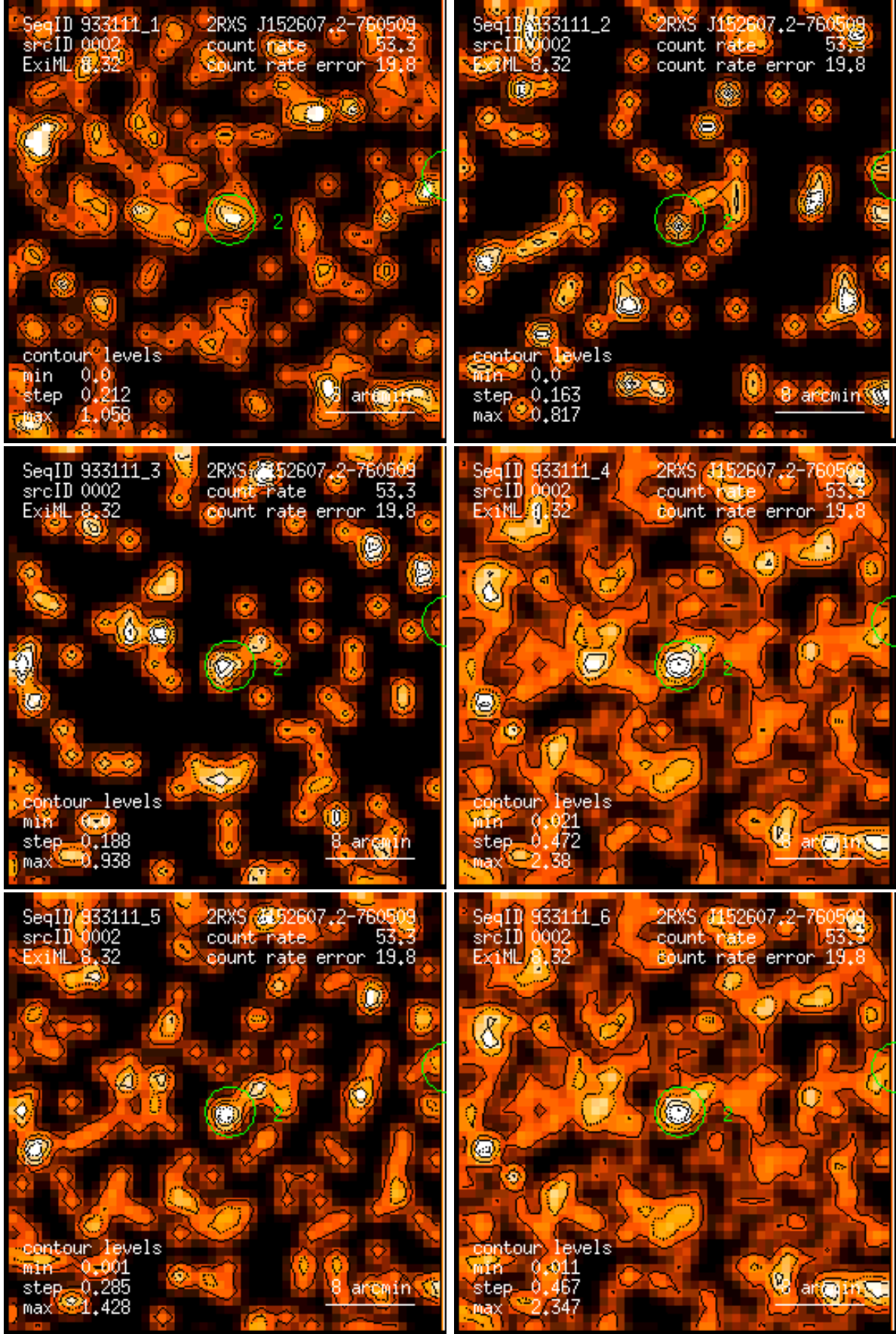
Figure 2: RASS 933111: detection 0002: band rate images, Gaussian filter: (1) PSPC channels 11 – 41, (2) 52 – 90, (3) 91 – 201, (4) 11 – 235, (5) 52 – 201, (6) 11 – 201. Broad band rates in counts/ks. Band rate contour levels in counts/ks/arcmin 2 .
