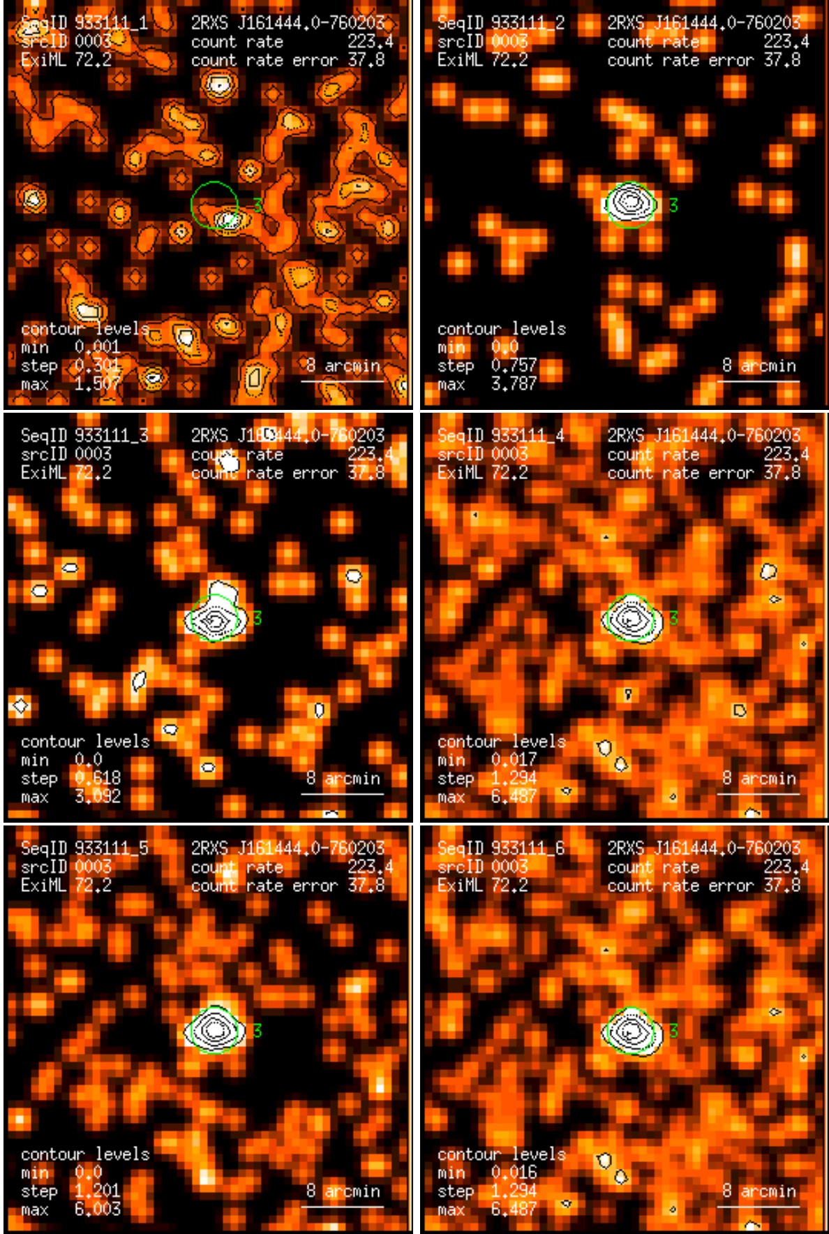
Figure 3: RASS 933111: detection 0003: band rate images, Gaussian filter: (1) PSPC channels 11 – 41, (2) 52 – 90, (3) 91 – 201, (4) 11 – 235, (5) 52 – 201, (6) 11 – 201. Broad band rates in counts/ks. Band rate contour levels in counts/ks/arcmin 2 .
