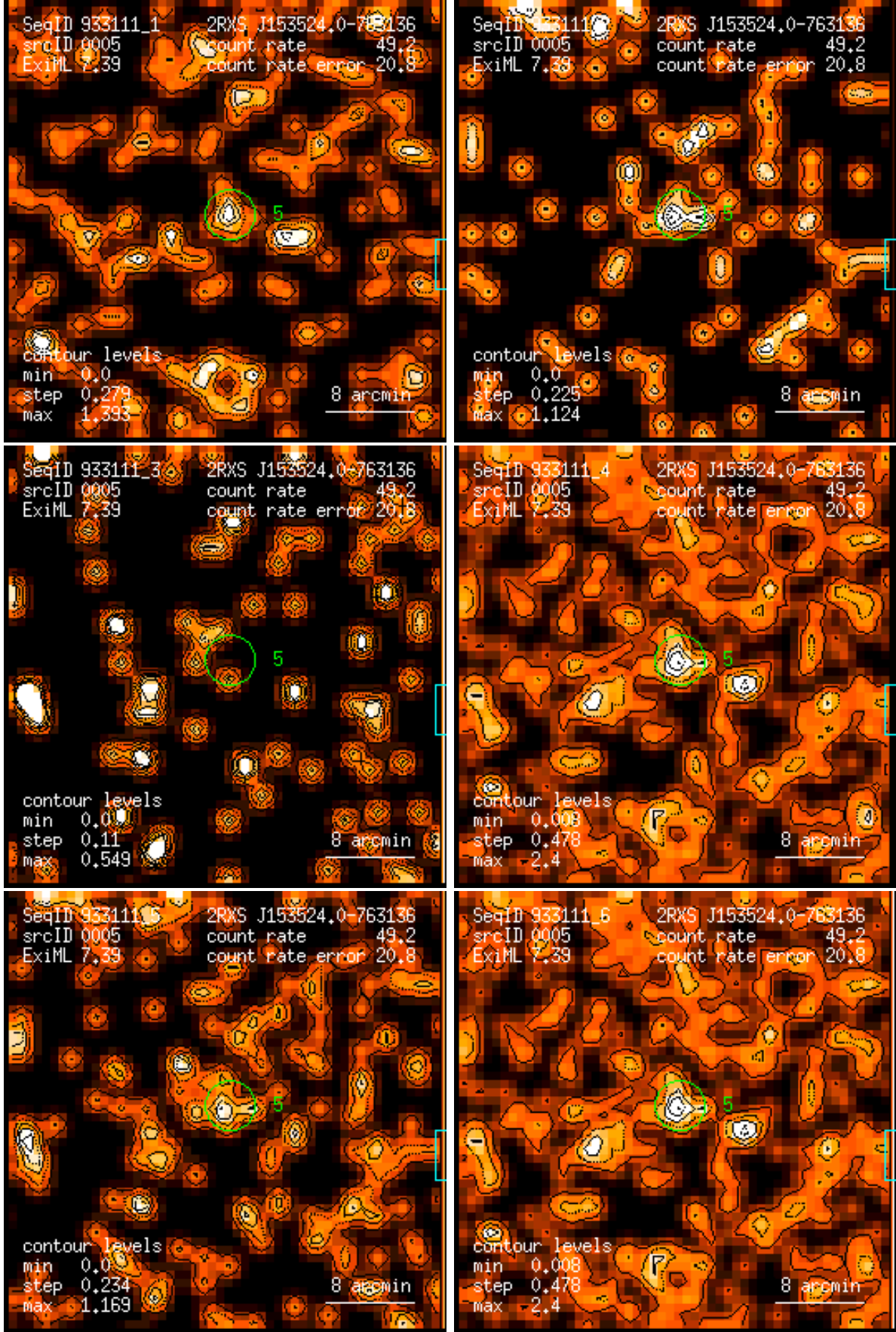
Figure 5: RASS 933111: detection 0005: band rate images, Gaussian filter: (1) PSPC channels 11 – 41, (2) 52 – 90, (3) 91 – 201, (4) 11 – 235, (5) 52 – 201, (6) 11 – 201. Broad band rates in counts/ks. Band rate contour levels in counts/ks/arcmin 2 .
