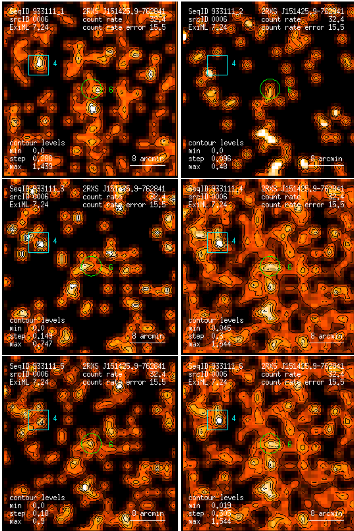
Figure 6: RASS 933111: detection 0006: band rate images, Gaussian filter: (1) PSPC channels 11 – 41, (2) 52 – 90, (3) 91 – 201, (4) 11 – 235, (5) 52 – 201, (6) 11 – 201. Broad band rates in counts/ks. Band rate contour levels in counts/ks/arcmin 2 .
