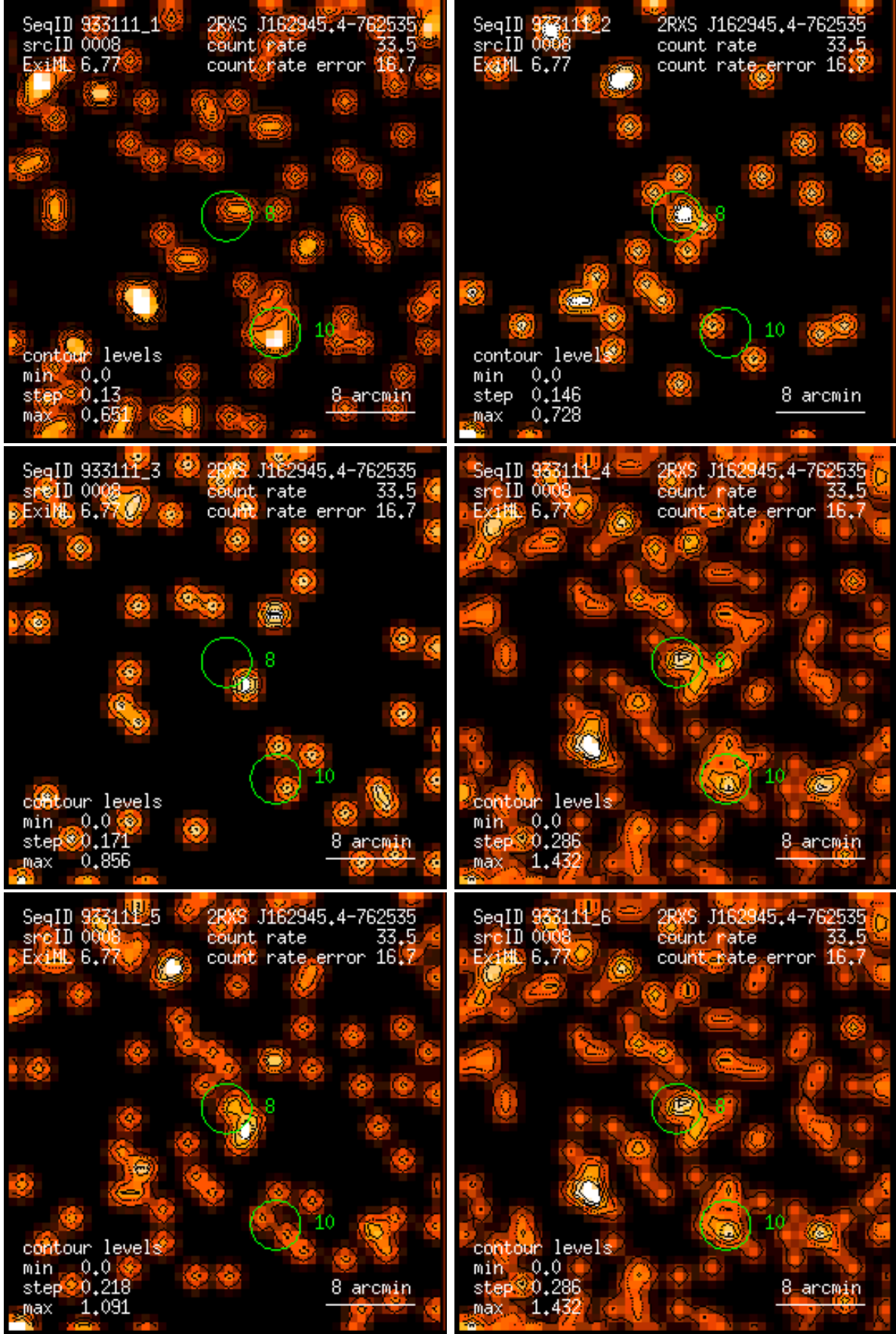
Figure 8: RASS 933111: detection 0008: band rate images, Gaussian filter: (1) PSPC channels 11 – 41, (2) 52 – 90, (3) 91 – 201, (4) 11 – 235, (5) 52 – 201, (6) 11 – 201. Broad band rates in counts/ks. Band rate contour levels in counts/ks/arcmin 2 .
