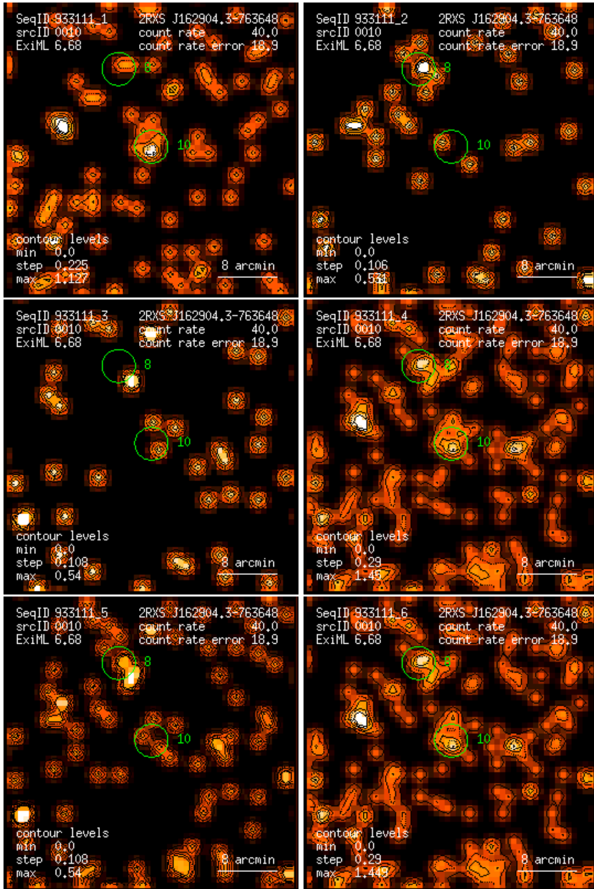
Figure 10: RASS 933111: detection 0010: band rate images, Gaussian filter: (1) PSPC channels 11 – 41, (2) 52 – 90, (3) 91 – 201, (4) 11 – 235, (5) 52 – 201, (6) 11 – 201. Broad band rates in counts/ks. Band rate contour levels in counts/ks/arcmin 2 .
