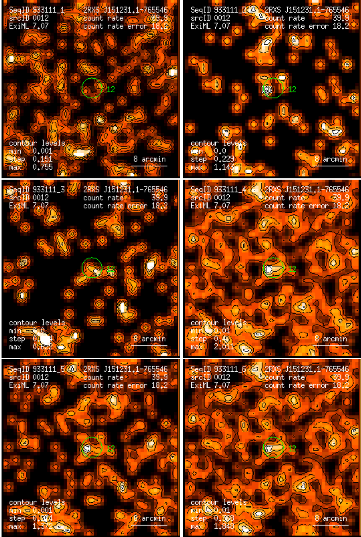
Figure 12: RASS 933111: detection 0012: band rate images, Gaussian filter: (1) PSPC channels 11 – 41, (2) 52 – 90, (3) 91 – 201, (4) 11 – 235, (5) 52 – 201, (6) 11 – 201. Broad band rates in counts/ks. Band rate contour levels in counts/ks/arcmin 2 .
