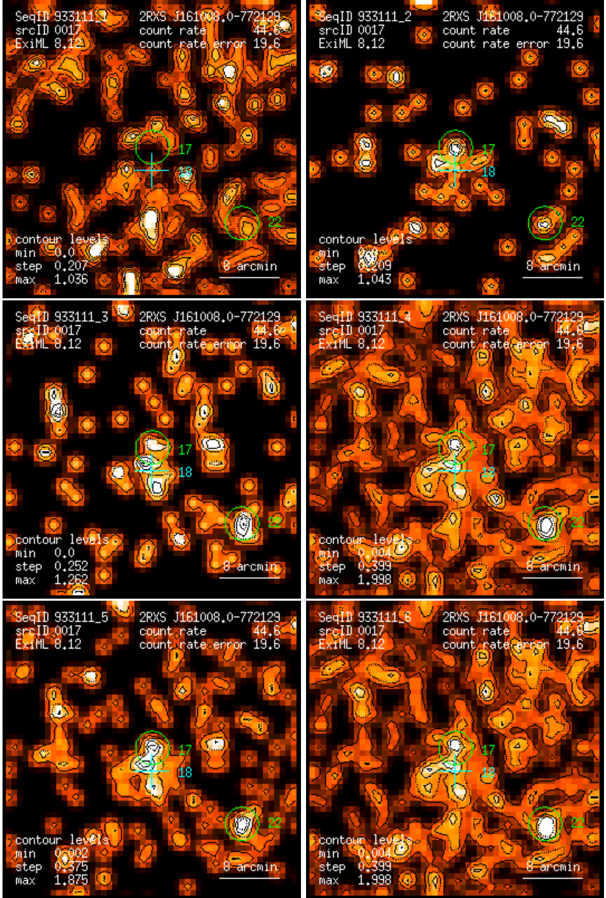
Figure 17: RASS 933111: detection 0017: band rate images, Gaussian filter: (1) PSPC channels 11 – 41, (2) 52 – 90, (3) 91 – 201, (4) 11 – 235, (5) 52 – 201, (6) 11 – 201. Broad band rates in counts/ks. Band rate contour levels in counts/ks/arcmin 2 .
