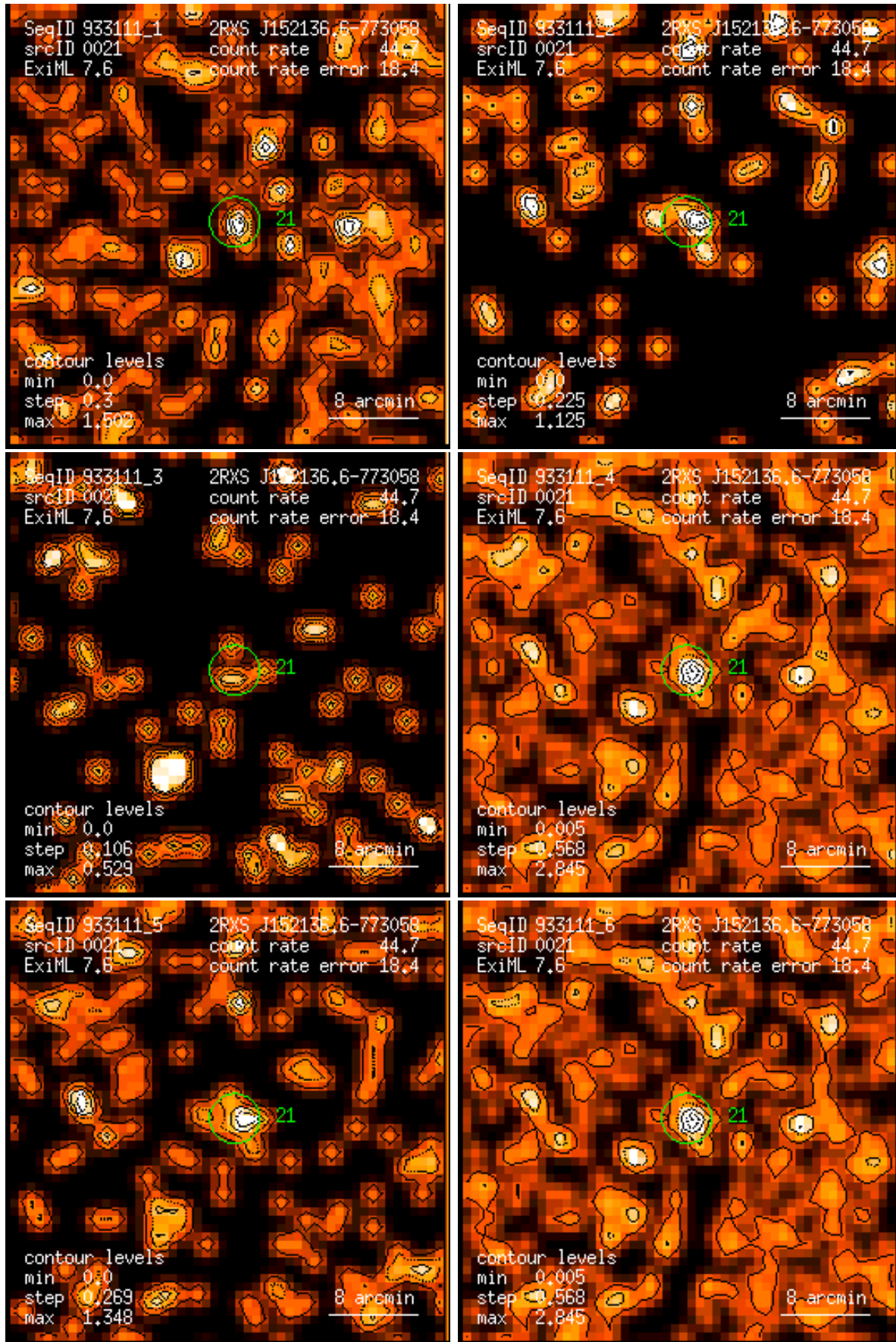
Figure 21: RASS 933111: detection 0021: band rate images, Gaussian filter: (1) PSPC channels 11 – 41, (2) 52 – 90, (3) 91 – 201, (4) 11 – 235, (5) 52 – 201, (6) 11 – 201. Broad band rates in counts/ks. Band rate contour levels in counts/ks/arcmin 2 .
