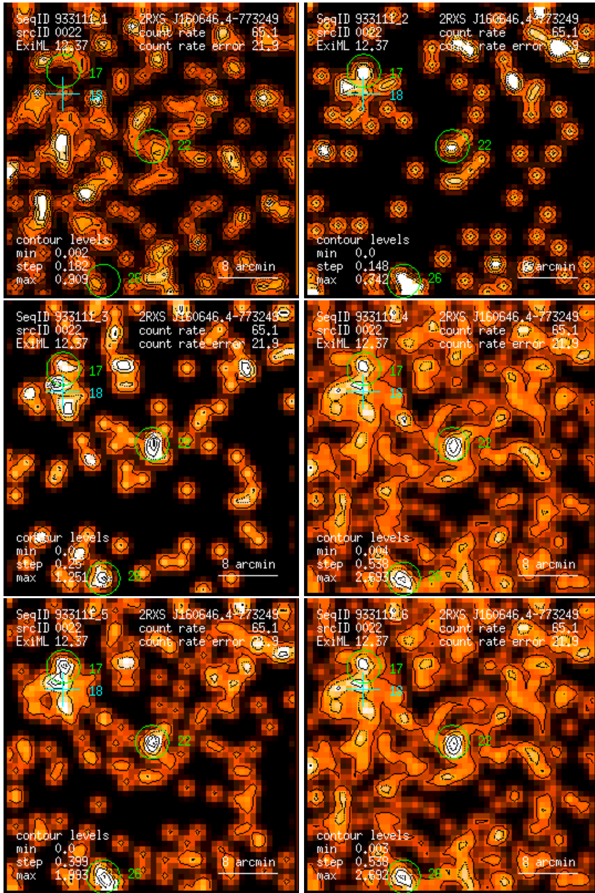
Figure 22: RASS 933111: detection 0022: band rate images, Gaussian filter: (1) PSPC channels 11 – 41, (2) 52 – 90, (3) 91 – 201, (4) 11 – 235, (5) 52 – 201, (6) 11 – 201. Broad band rates in counts/ks. Band rate contour levels in counts/ks/arcmin 2 .
