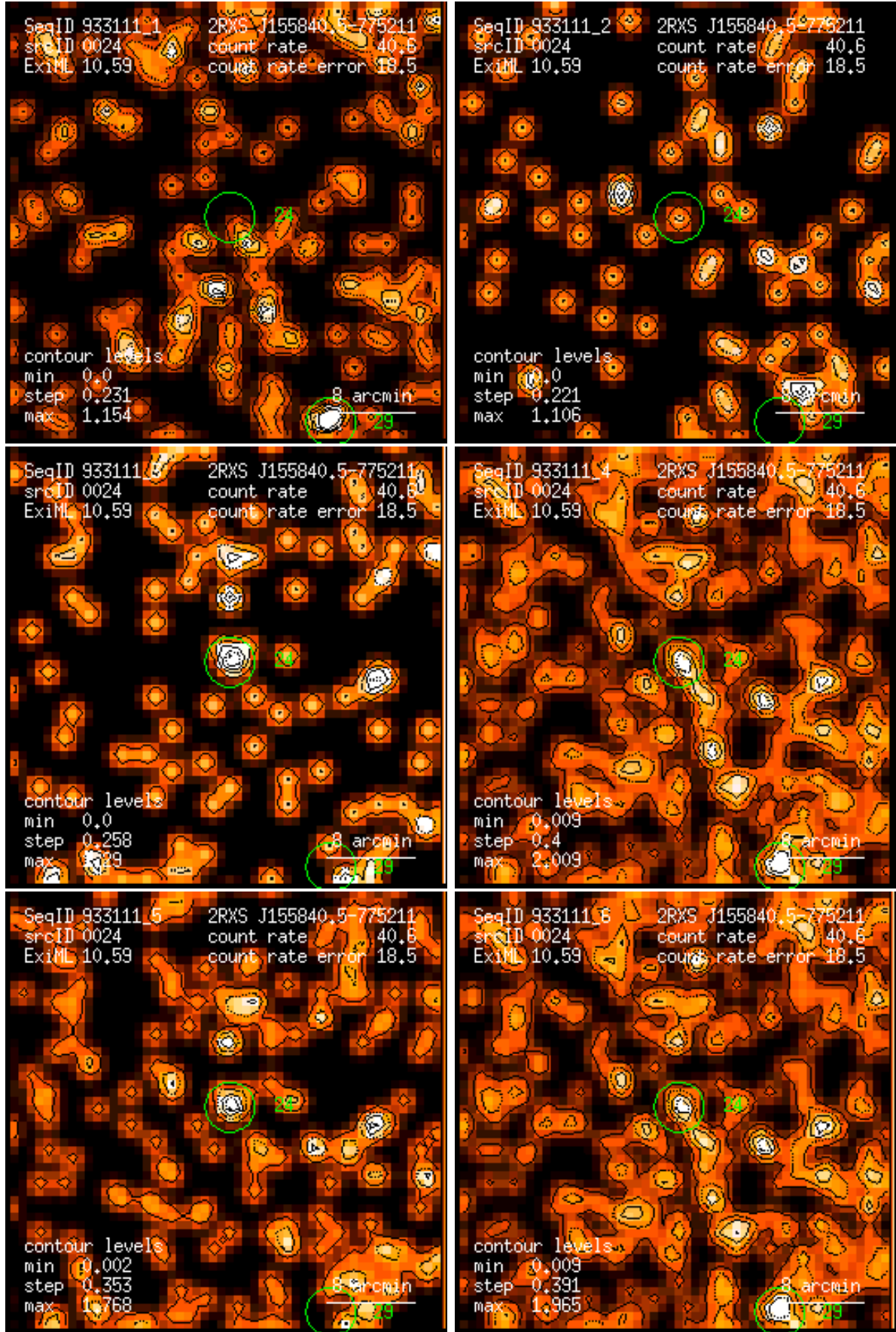
Figure 24: RASS 933111: detection 0024: band rate images, Gaussian filter: (1) PSPC channels 11 – 41, (2) 52 – 90, (3) 91 – 201, (4) 11 – 235, (5) 52 – 201, (6) 11 – 201. Broad band rates in counts/ks. Band rate contour levels in counts/ks/arcmin 2 .
