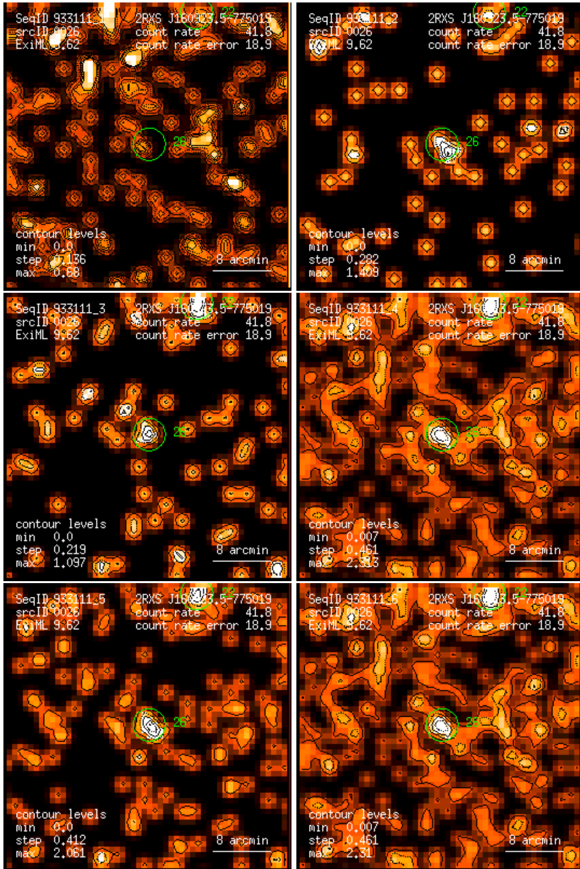
Figure 26: RASS 933111: detection 0026: band rate images, Gaussian filter: (1) PSPC channels 11 – 41, (2) 52 – 90, (3) 91 – 201, (4) 11 – 235, (5) 52 – 201, (6) 11 – 201. Broad band rates in counts/ks. Band rate contour levels in counts/ks/arcmin 2 .
