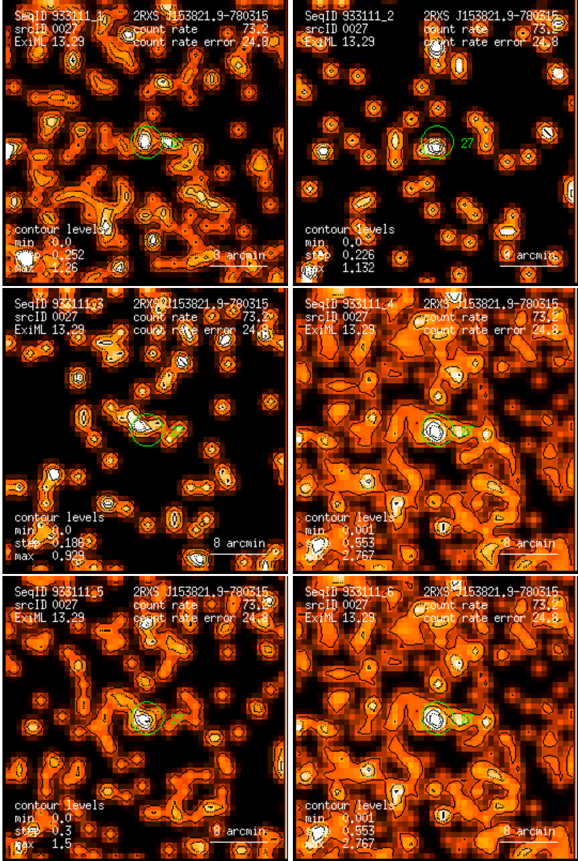
Figure 27: RASS 933111: detection 0027: band rate images, Gaussian filter: (1) PSPC channels 11 – 41, (2) 52 – 90, (3) 91 – 201, (4) 11 – 235, (5) 52 – 201, (6) 11 – 201. Broad band rates in counts/ks. Band rate contour levels in counts/ks/arcmin 2 .
