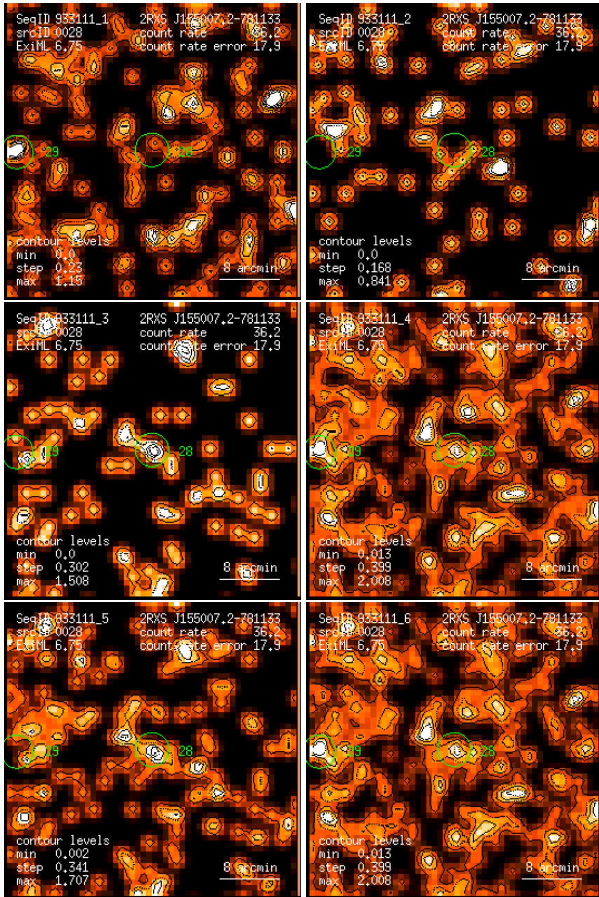
Figure 28: RASS 933111: detection 0028: band rate images, Gaussian filter: (1) PSPC channels 11 – 41, (2) 52 – 90, (3) 91 – 201, (4) 11 – 235, (5) 52 – 201, (6) 11 – 201. Broad band rates in counts/ks. Band rate contour levels in counts/ks/arcmin 2 .
