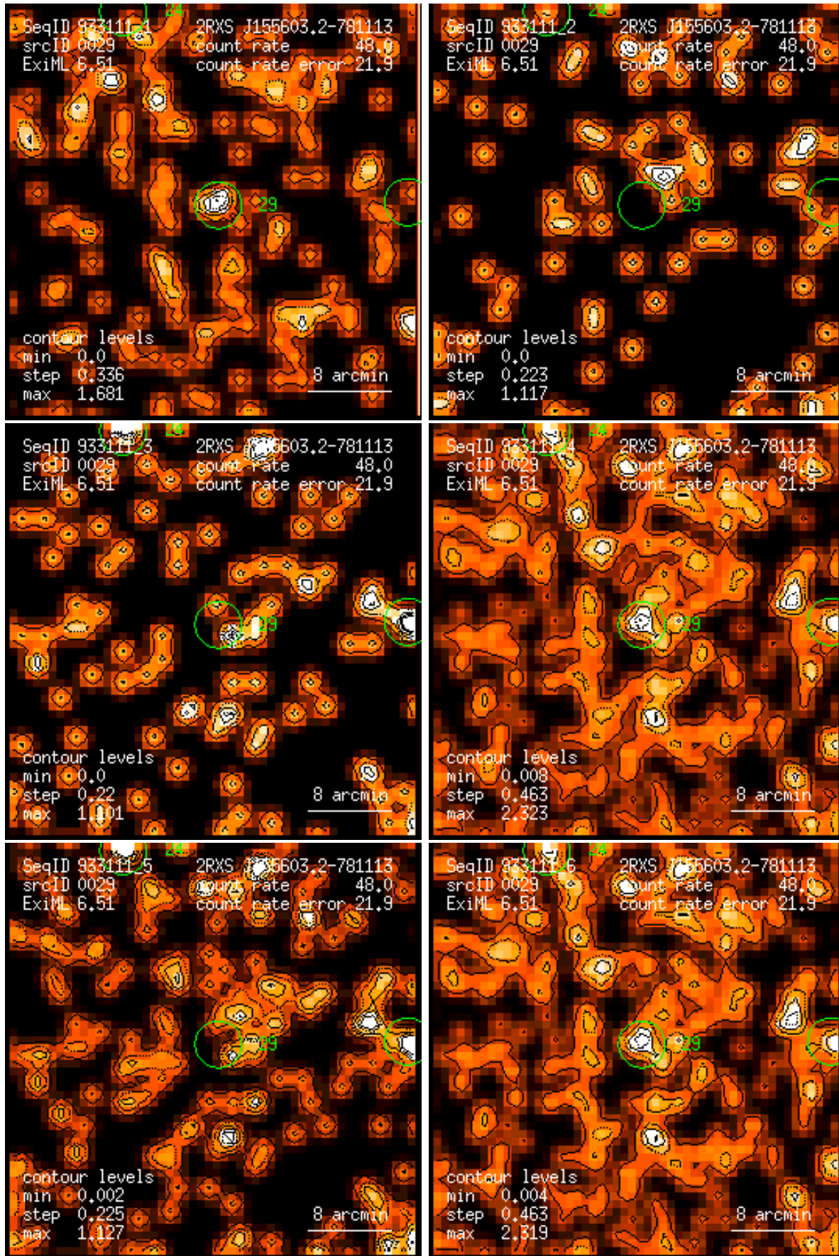
Figure 29: RASS 933111: detection 0029: band rate images, Gaussian filter: (1) PSPC channels 11 – 41, (2) 52 – 90, (3) 91 – 201, (4) 11 – 235, (5) 52 – 201, (6) 11 – 201. Broad band rates in counts/ks. Band rate contour levels in counts/ks/arcmin 2 .
