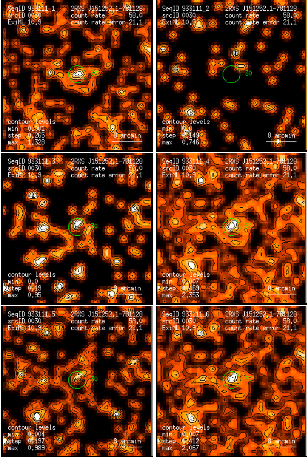
Figure 30: RASS 933111: detection 0030: band rate images, Gaussian filter: (1) PSPC channels 11 – 41, (2) 52 – 90, (3) 91 – 201, (4) 11 – 235, (5) 52 – 201, (6) 11 – 201. Broad band rates in counts/ks. Band rate contour levels in counts/ks/arcmin 2 .
