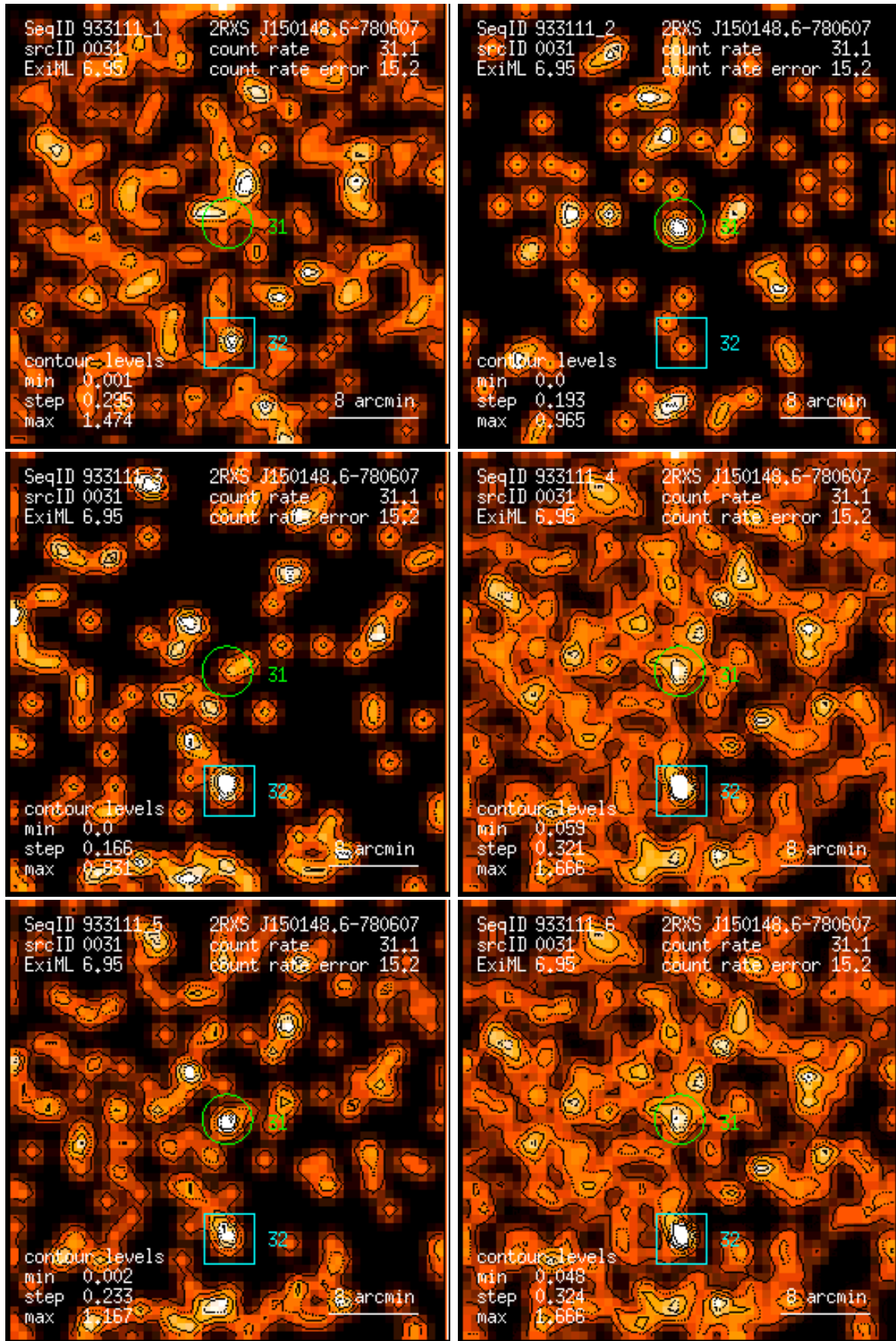
Figure 31: RASS 933111: detection 0031: band rate images, Gaussian filter: (1) PSPC channels 11 – 41, (2) 52 – 90, (3) 91 – 201, (4) 11 – 235, (5) 52 – 201, (6) 11 – 201. Broad band rates in counts/ks. Band rate contour levels in counts/ks/arcmin 2 .
