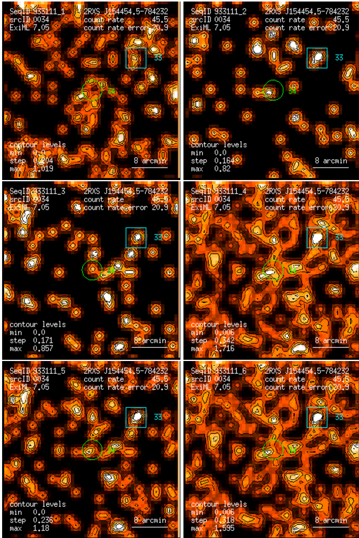
Figure 34: RASS 933111: detection 0034: band rate images, Gaussian filter: (1) PSPC channels 11 – 41, (2) 52 – 90, (3) 91 – 201, (4) 11 – 235, (5) 52 – 201, (6) 11 – 201. Broad band rates in counts/ks. Band rate contour levels in counts/ks/arcmin 2 .
