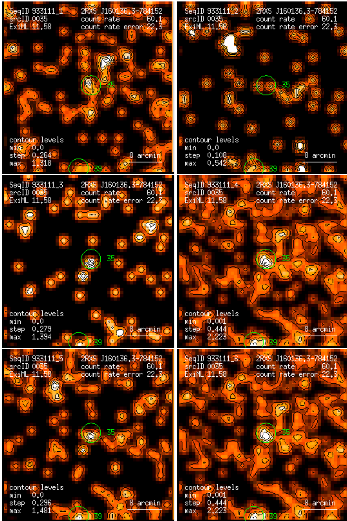
Figure 35: RASS 933111: detection 0035: band rate images, Gaussian filter: (1) PSPC channels 11 – 41, (2) 52 – 90, (3) 91 – 201, (4) 11 – 235, (5) 52 – 201, (6) 11 – 201. Broad band rates in counts/ks. Band rate contour levels in counts/ks/arcmin 2 .
