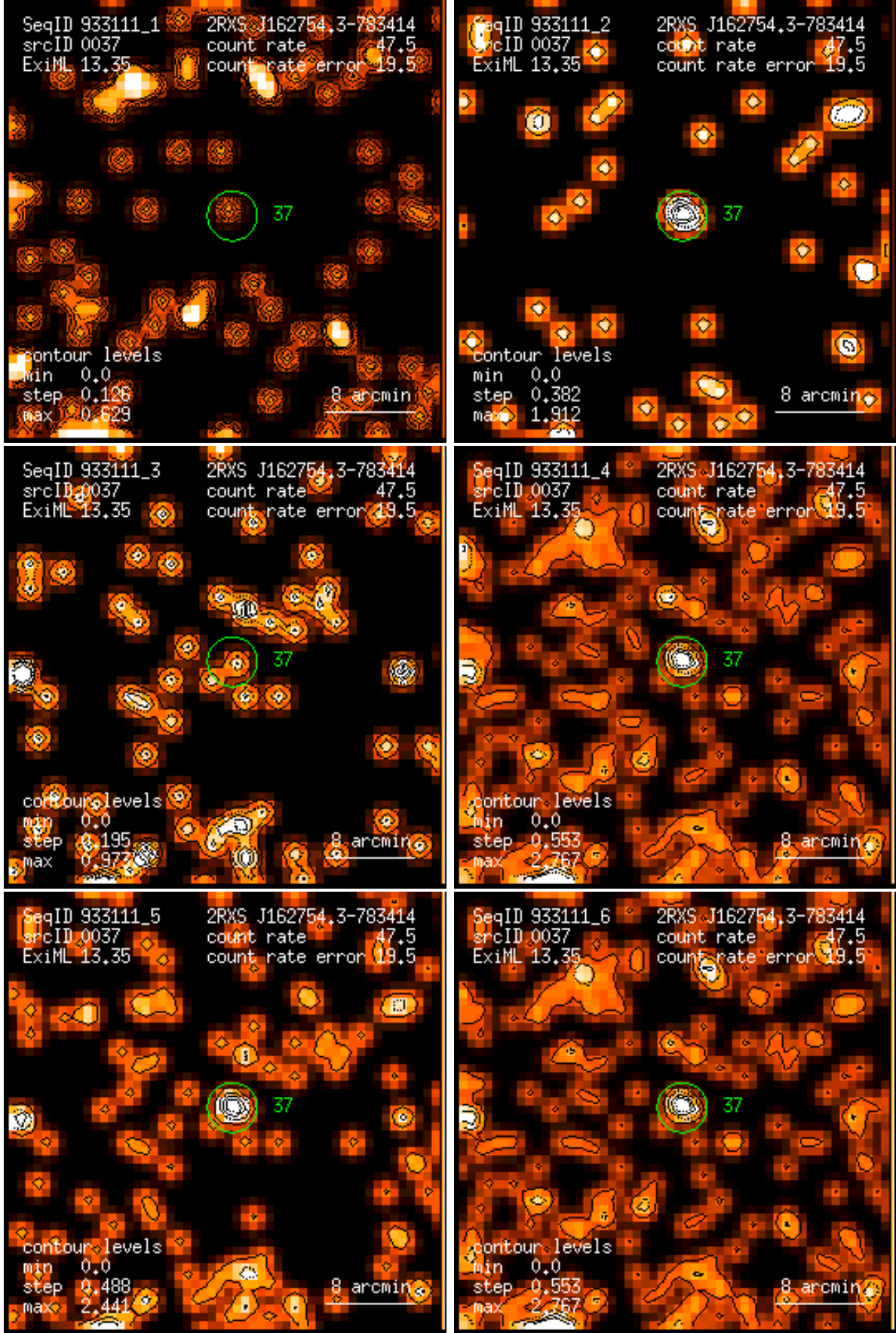
Figure 37: RASS 933111: detection 0037: band rate images, Gaussian filter: (1) PSPC channels 11 – 41, (2) 52 – 90, (3) 91 – 201, (4) 11 – 235, (5) 52 – 201, (6) 11 – 201. Broad band rates in counts/ks. Band rate contour levels in counts/ks/arcmin 2 .
