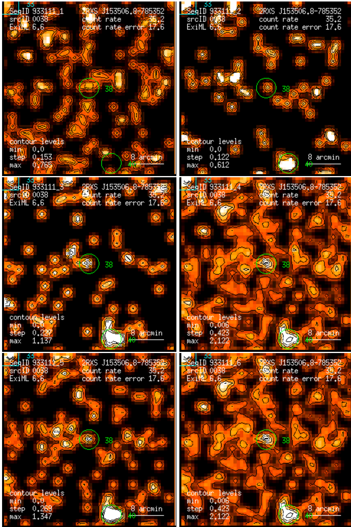
Figure 38: RASS 933111: detection 0038: band rate images, Gaussian filter: (1) PSPC channels 11 – 41, (2) 52 – 90, (3) 91 – 201, (4) 11 – 235, (5) 52 – 201, (6) 11 – 201. Broad band rates in counts/ks. Band rate contour levels in counts/ks/arcmin 2 .
