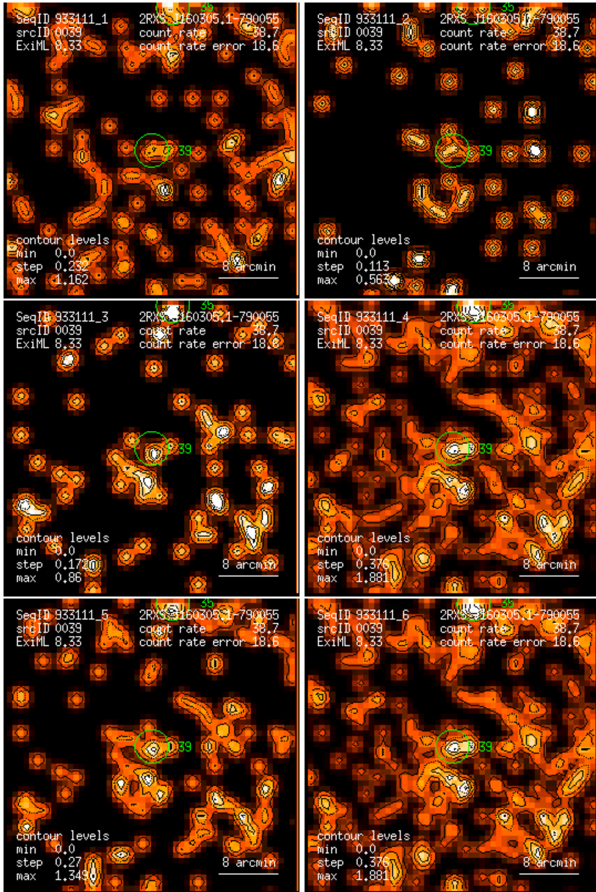
Figure 39: RASS 933111: detection 0039: band rate images, Gaussian filter: (1) PSPC channels 11 – 41, (2) 52 – 90, (3) 91 – 201, (4) 11 – 235, (5) 52 – 201, (6) 11 – 201. Broad band rates in counts/ks. Band rate contour levels in counts/ks/arcmin 2 .
