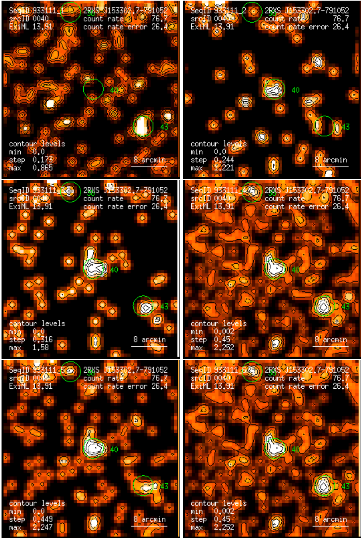
Figure 40: RASS 933111: detection 0040: band rate images, Gaussian filter: (1) PSPC channels 11 – 41, (2) 52 – 90, (3) 91 – 201, (4) 11 – 235, (5) 52 – 201, (6) 11 – 201. Broad band rates in counts/ks. Band rate contour levels in counts/ks/arcmin 2 .
