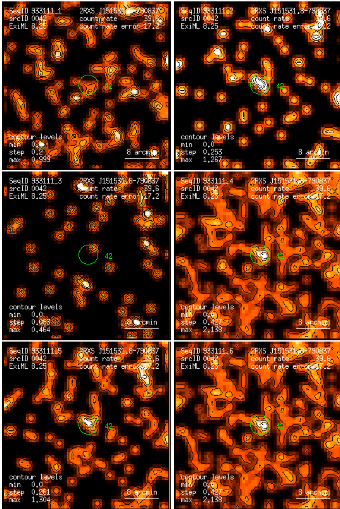
Figure 42: RASS 933111: detection 0042: band rate images, Gaussian filter: (1) PSPC channels 11 – 41, (2) 52 – 90, (3) 91 – 201, (4) 11 – 235, (5) 52 – 201, (6) 11 – 201. Broad band rates in counts/ks. Band rate contour levels in counts/ks/arcmin 2 .
