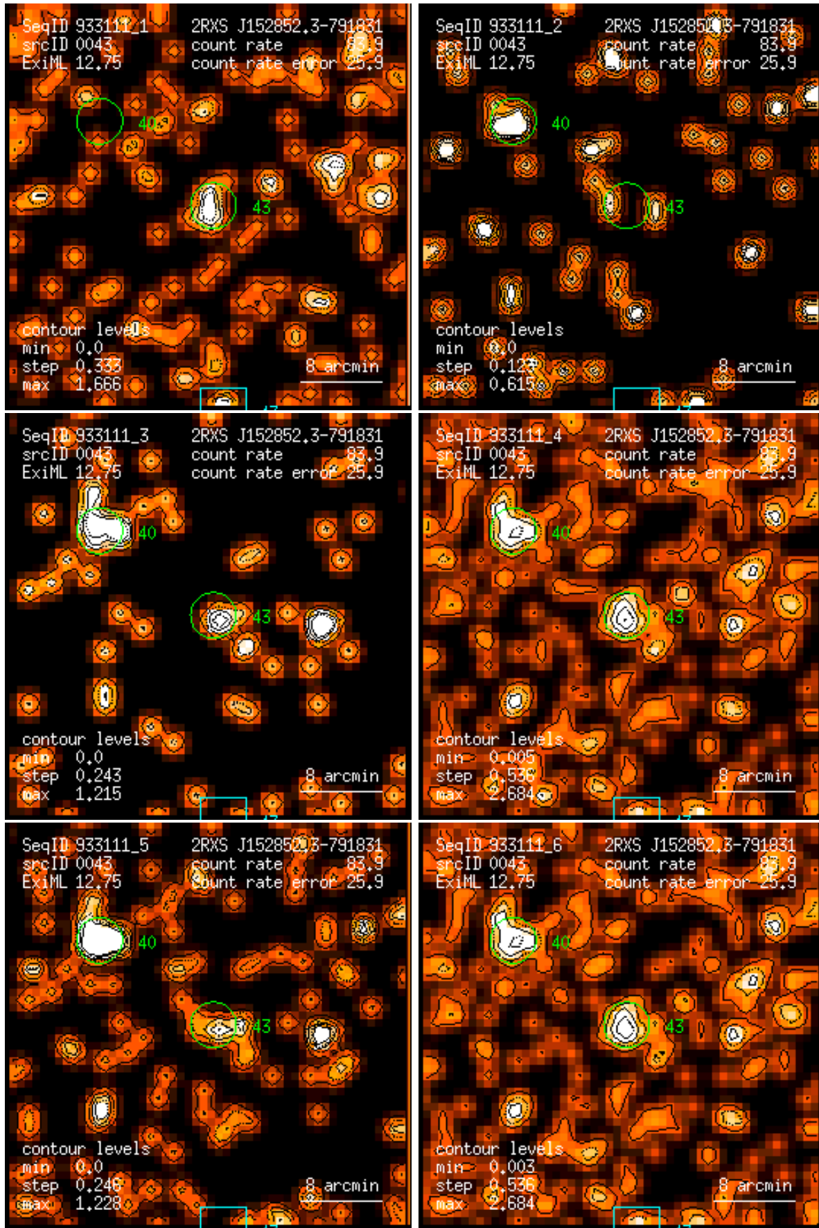
Figure 43: RASS 933111: detection 0043: band rate images, Gaussian filter: (1) PSPC channels 11 – 41, (2) 52 – 90, (3) 91 – 201, (4) 11 – 235, (5) 52 – 201, (6) 11 – 201. Broad band rates in counts/ks. Band rate contour levels in counts/ks/arcmin 2 .
