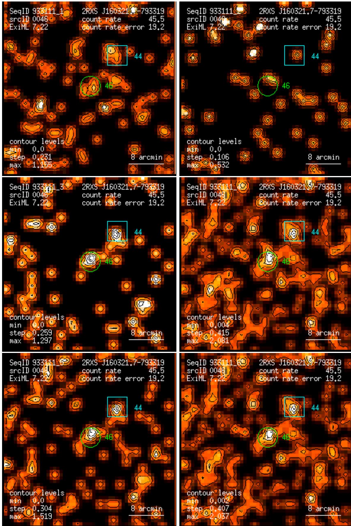
Figure 46: RASS 933111: detection 0046: band rate images, Gaussian filter: (1) PSPC channels 11 – 41, (2) 52 – 90, (3) 91 – 201, (4) 11 – 235, (5) 52 – 201, (6) 11 – 201. Broad band rates in counts/ks. Band rate contour levels in counts/ks/arcmin 2 .
